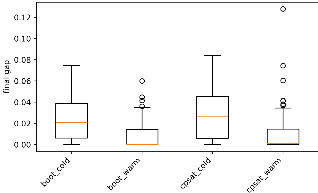
Final gap by method
