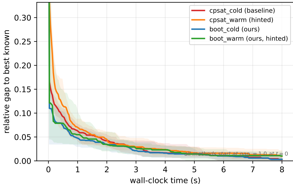
Anytime solution quality — job-shop 15x15 (median over held-out stream instances, IQR band)
