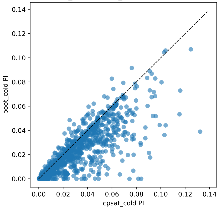
cpsat_cold vs boot_cold: primal integral
