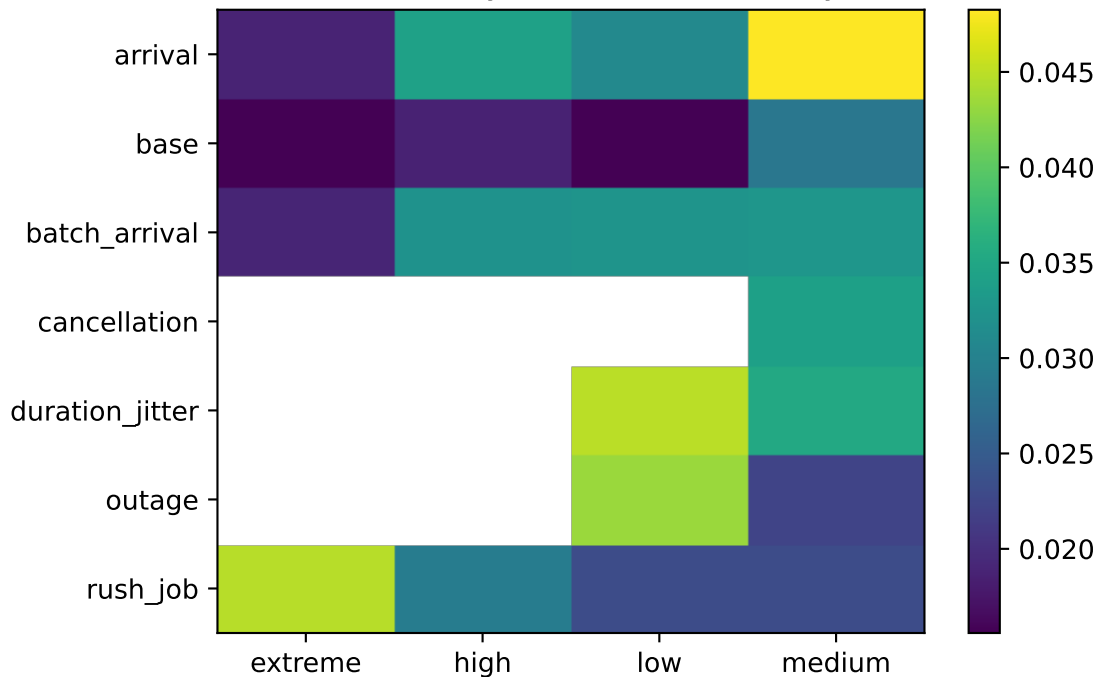
Median PI by delta kind x severity
