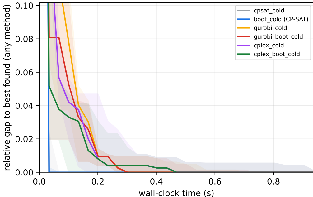
Anytime quality — job-shop, cross-solver (median over held-out stream instances, IQR band)
