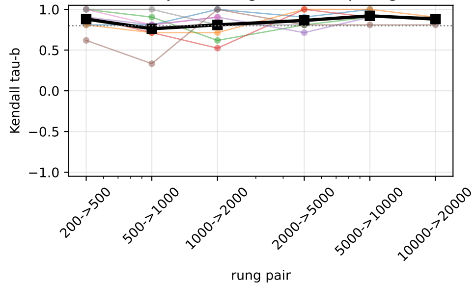
Kendall tau, adjacent rungs: all 7 competing methods
