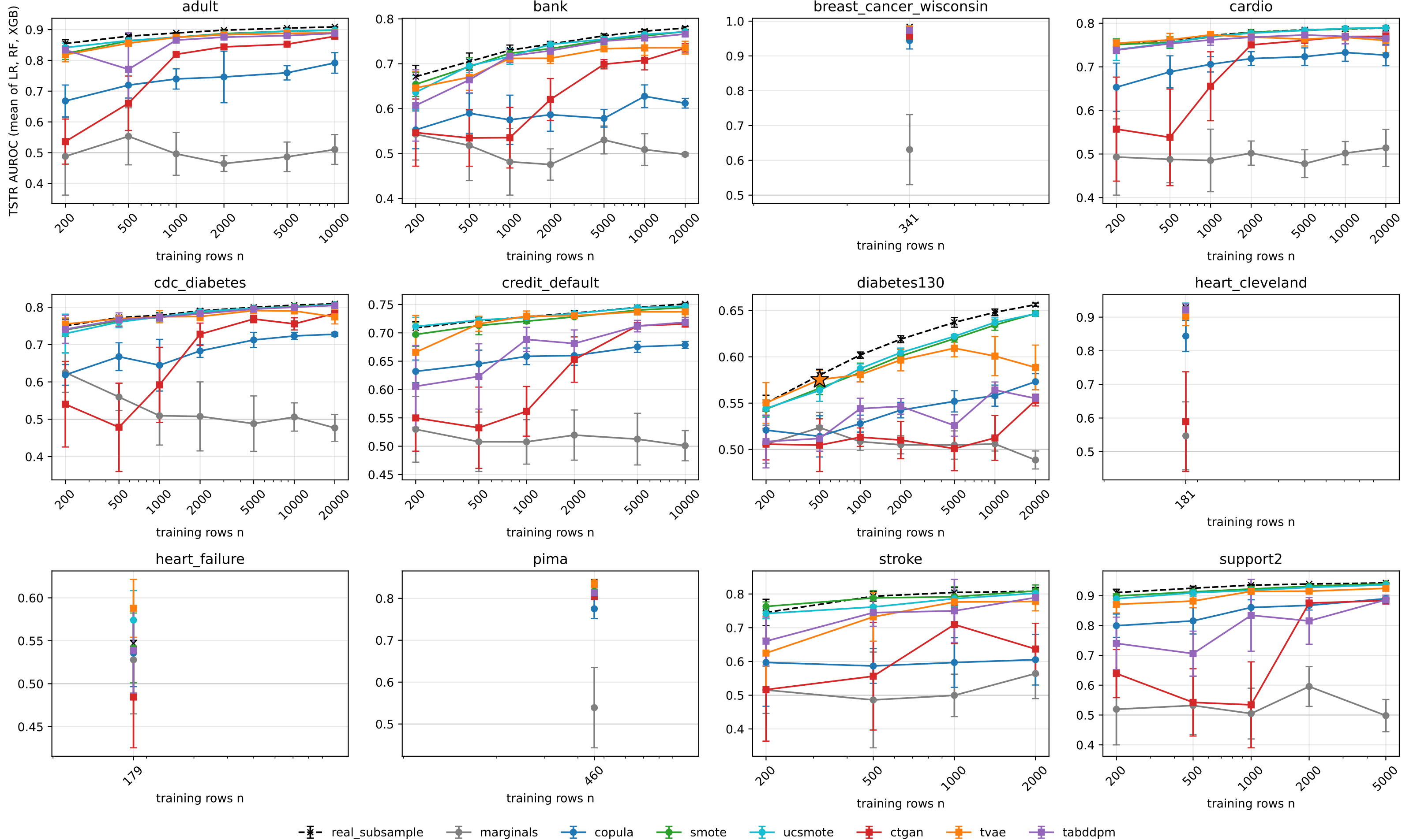
Utility against training size; error bars = std over seeds; star = crossover (analysis 1)
