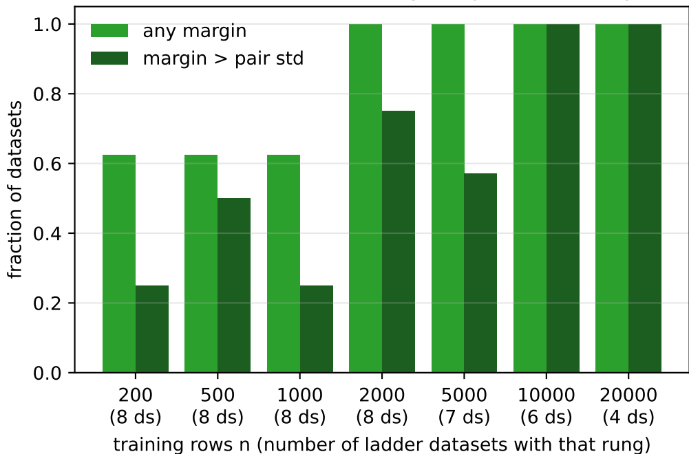
Best trivial baseline beats every deep model (analysis 2)
