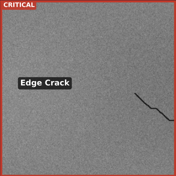
Dicing stress / handling
