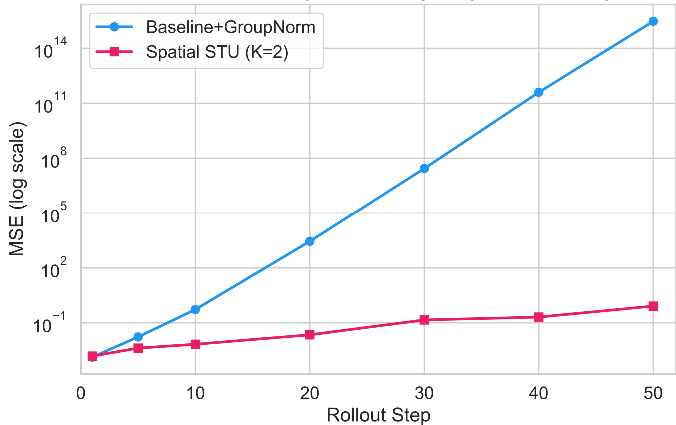
Rollout Error Divergence — Pong, Single-Step Training
