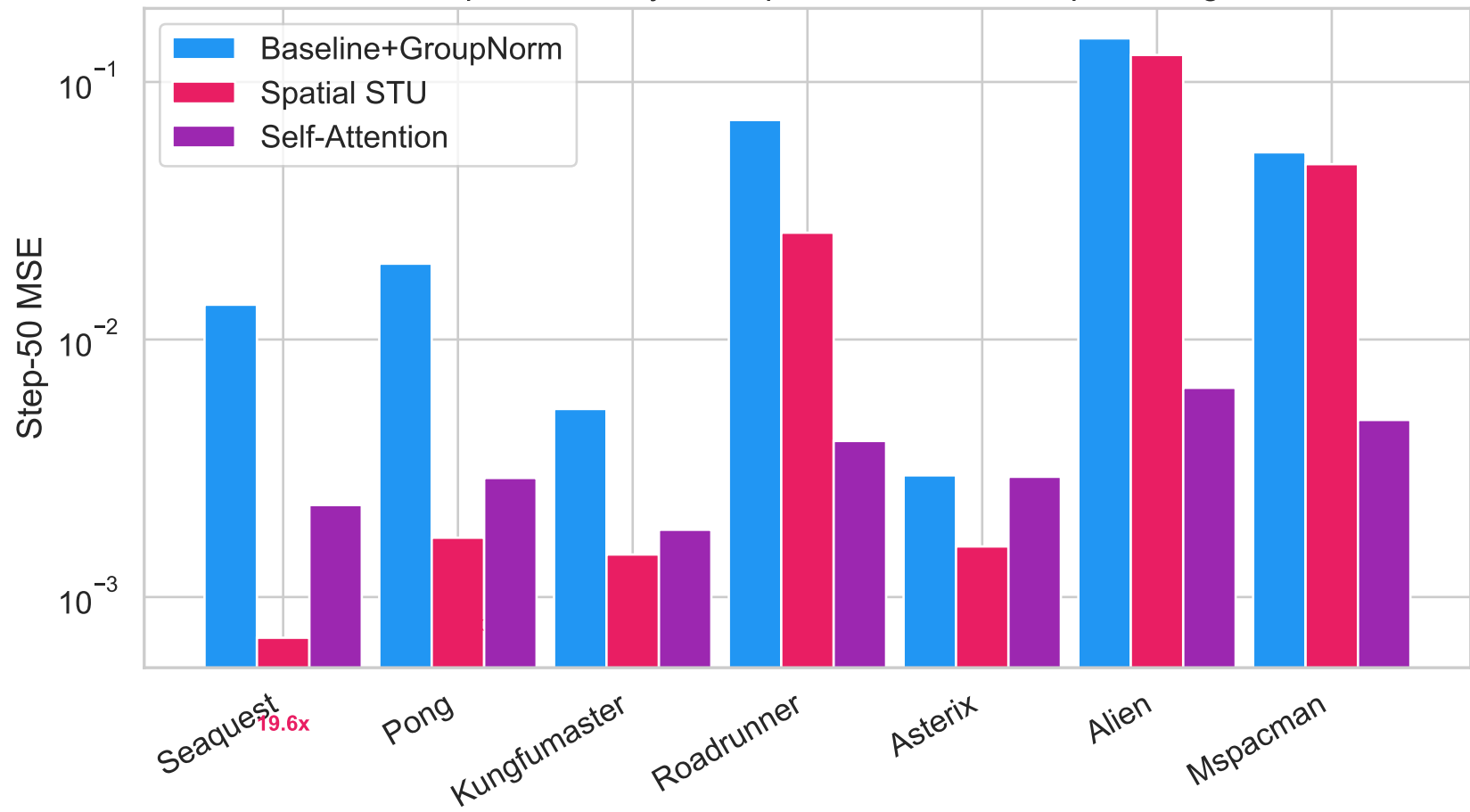
Sample Efficiency at 5 Episodes — Multi-Step Training
