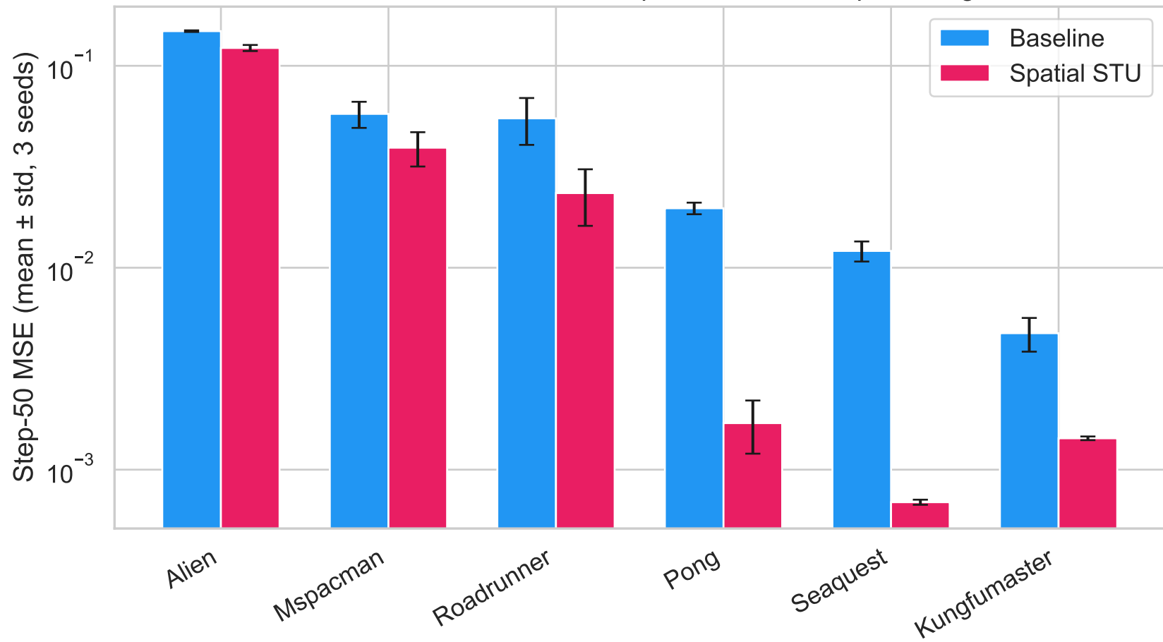
Multi-Seed Validation — 5 Episodes, Multi-Step Training
