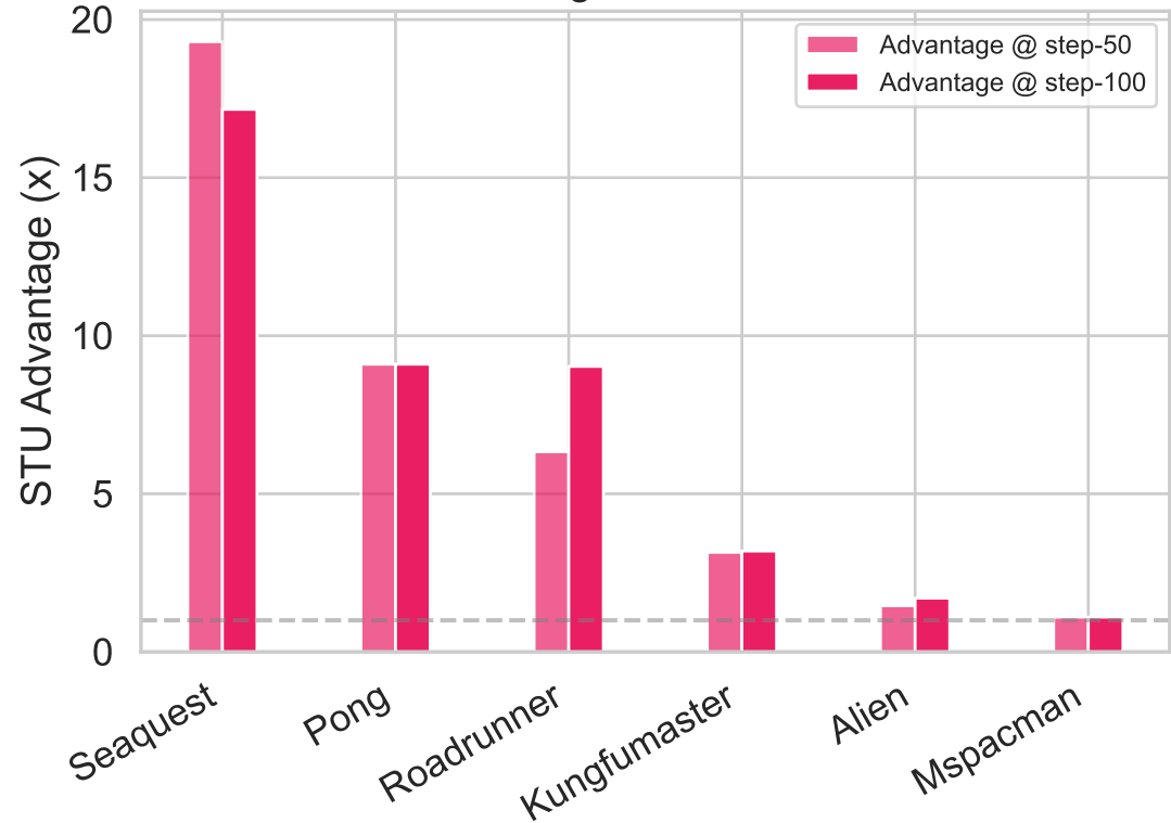
STU Advantage Grows with Horizon
