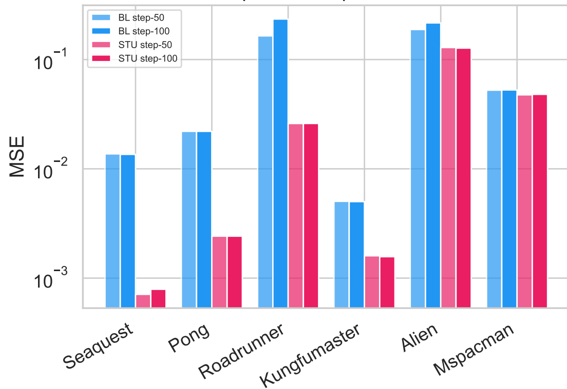
Step-50 vs Step-100 MSE
