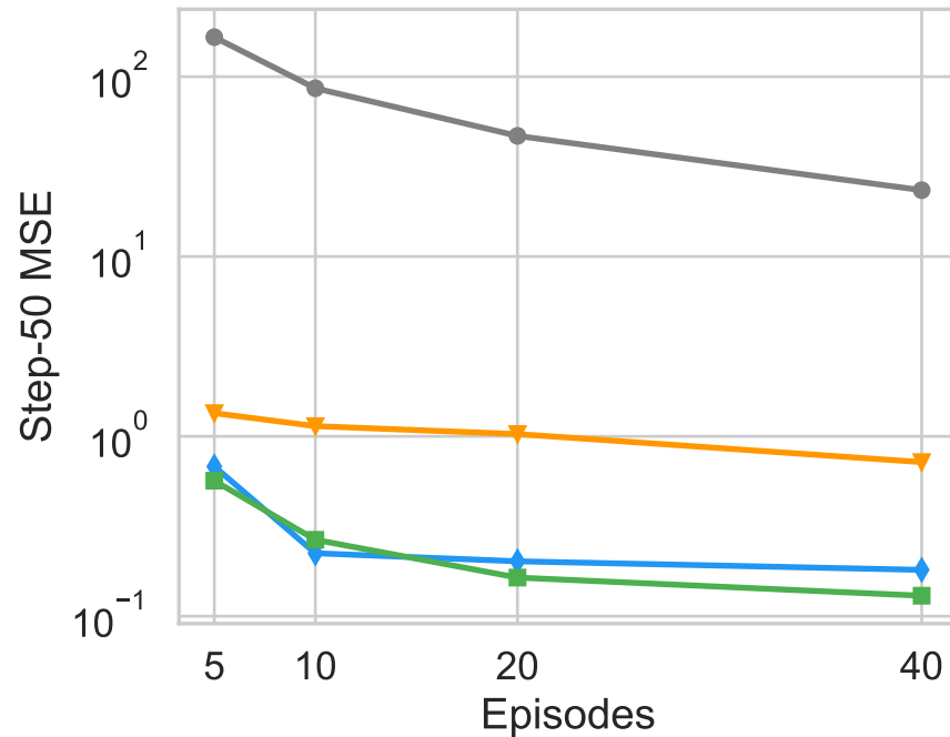
Walker Walk
