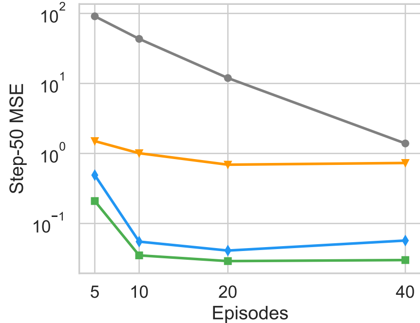
Cheetah Run
