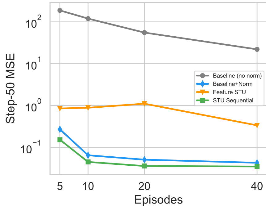
Hopper Hop
