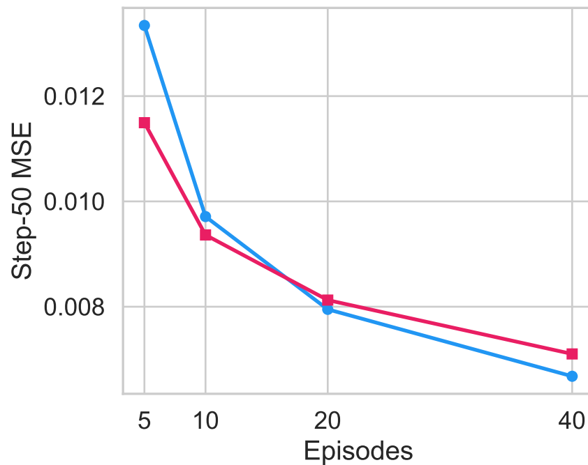
Walker Walk
