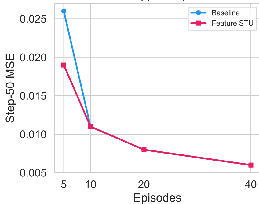
Hopper Hop
