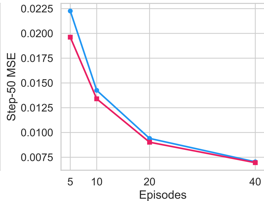
Cheetah Run
