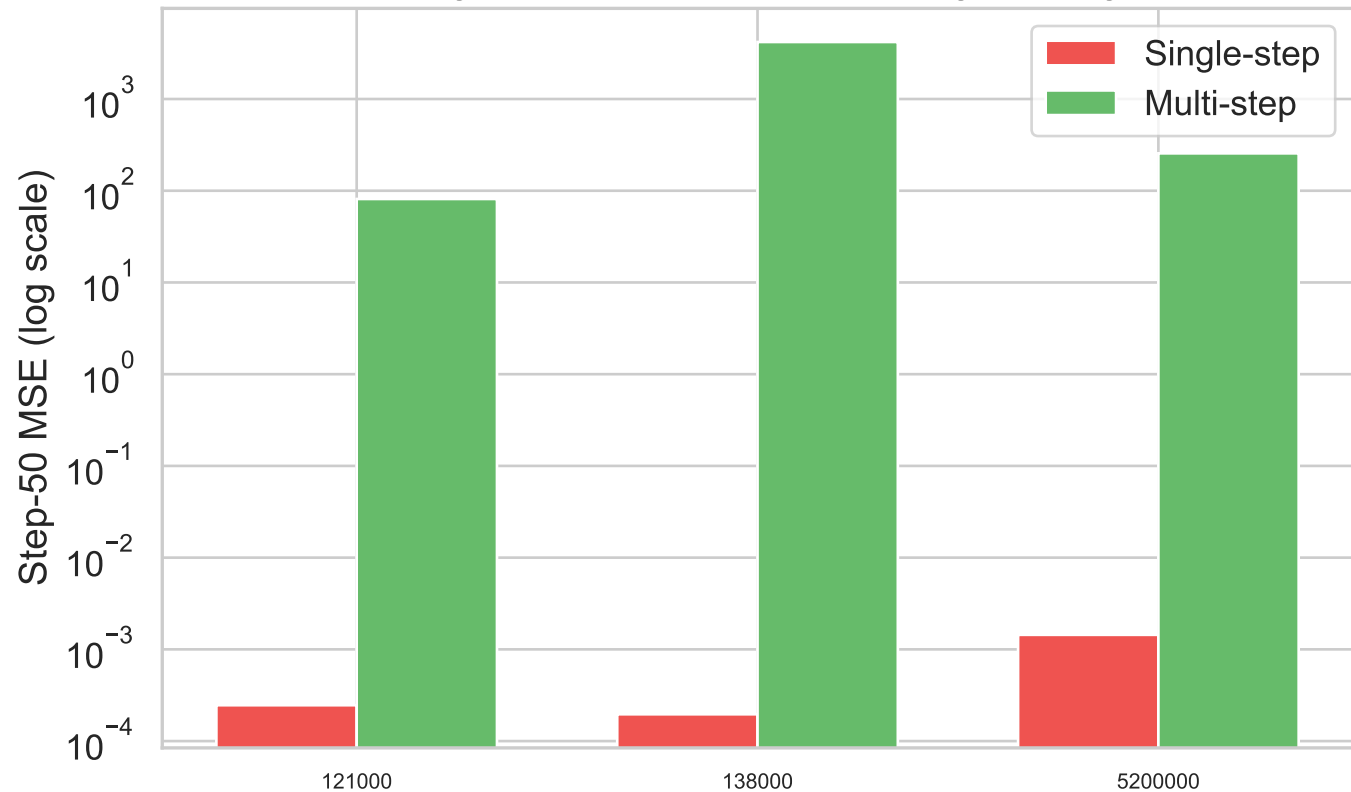
Single-Step vs Multi-Step Training — Pong
