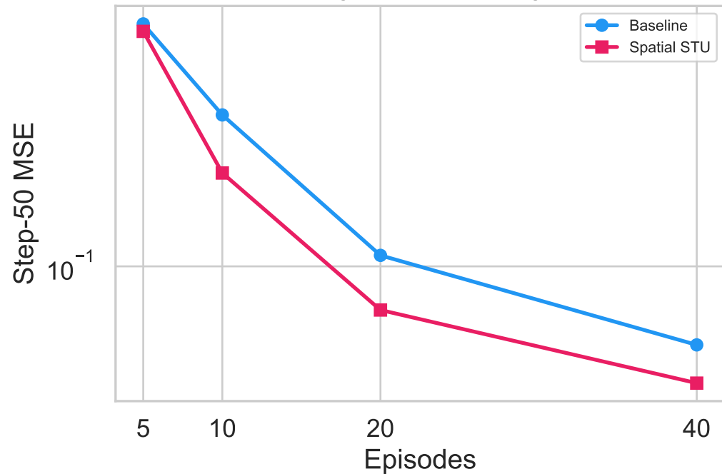
Single-Step Training
