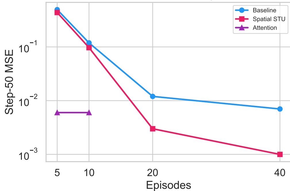
Multi-Step Training
