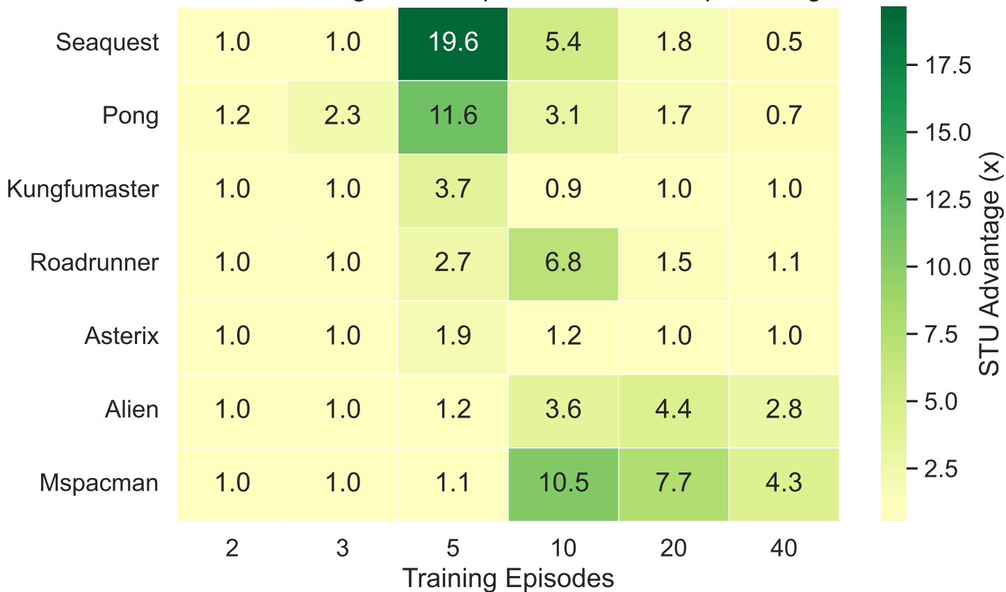
STU Advantage Heatmap — Atari Multi-Step Training
