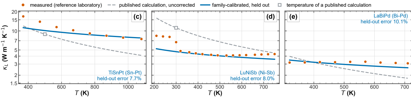
(c)–(e): three best of 21 eligible held-out fits ( \geq 25 temperatures over \geq 300 K); median over all 21: 21.7%
