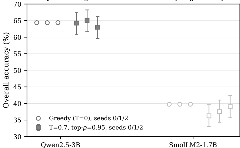
Greedy decoding is seed-invariant; sampling adds spread
