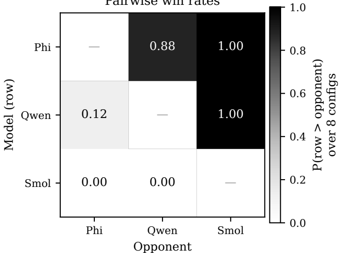
Pairwise win rates
