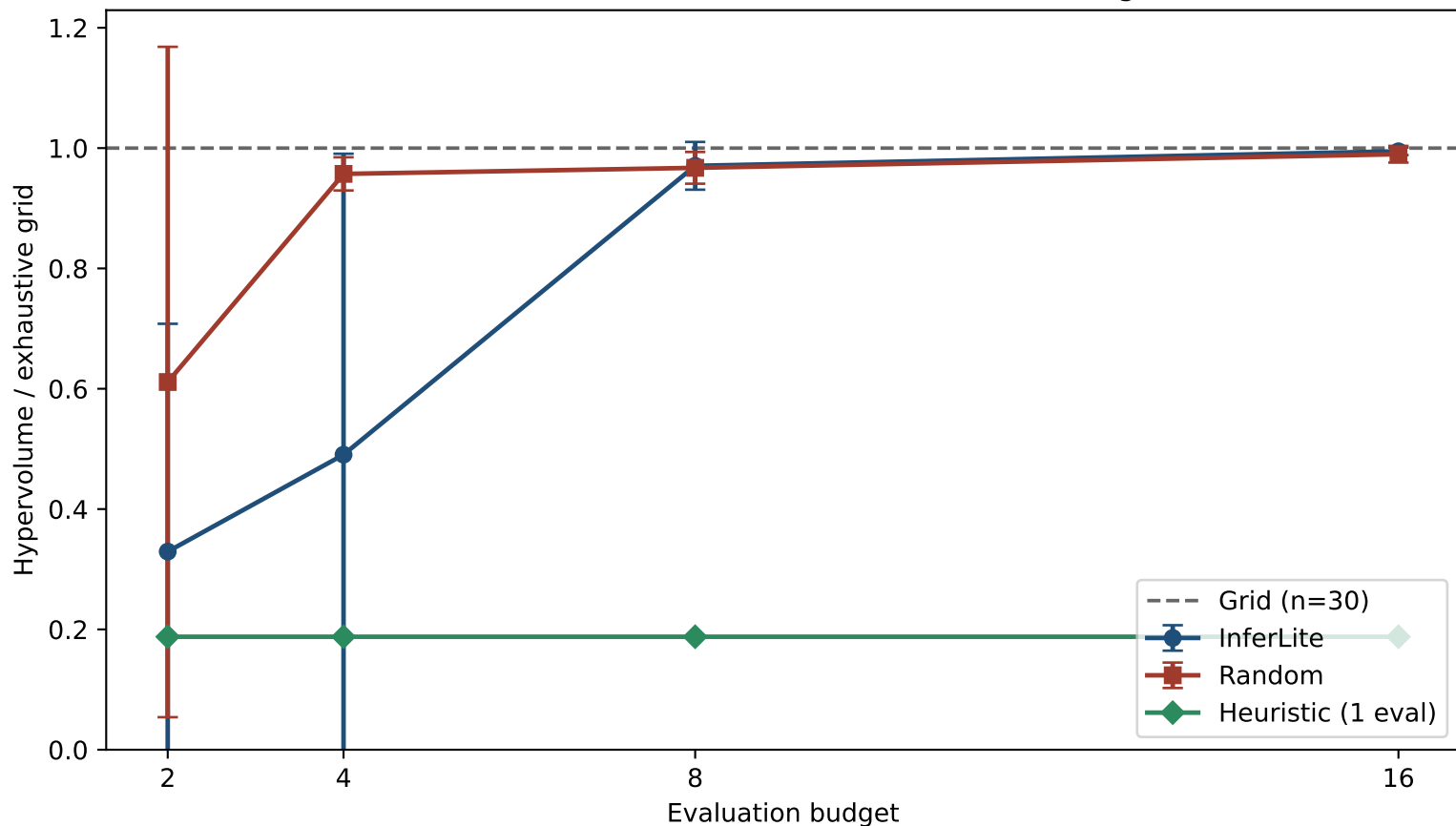
Does InferLite reach a good Pareto front faster than random search? 5 seeds, 95% t-interval, n=30 measured configs
