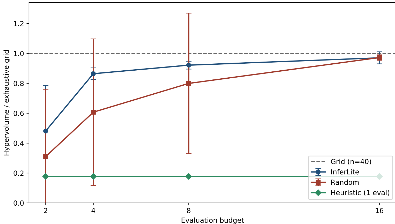
Does InferLite reach a good Pareto front faster than random search? 5 seeds, 95% t-interval, n=40 measured configs
