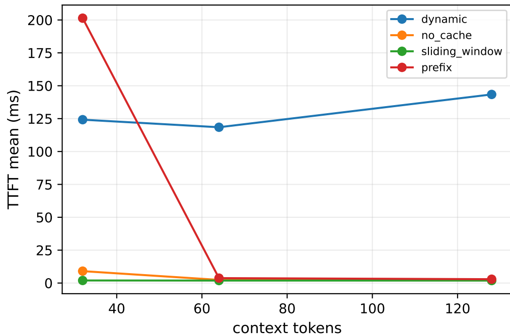
Prefill vs context
