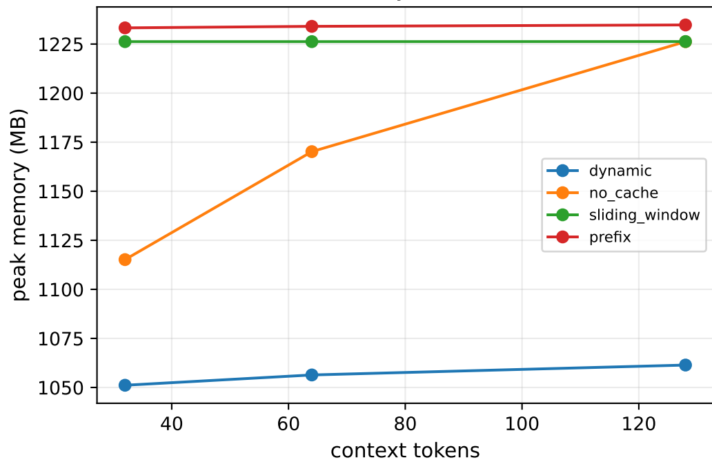
KV memory vs context
