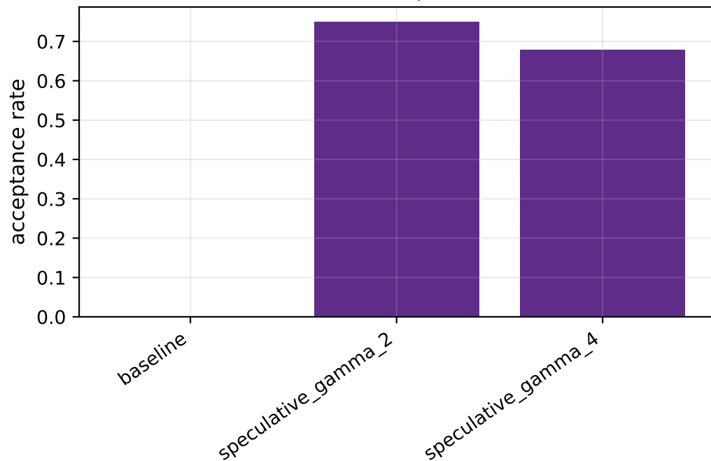
Draft acceptance
