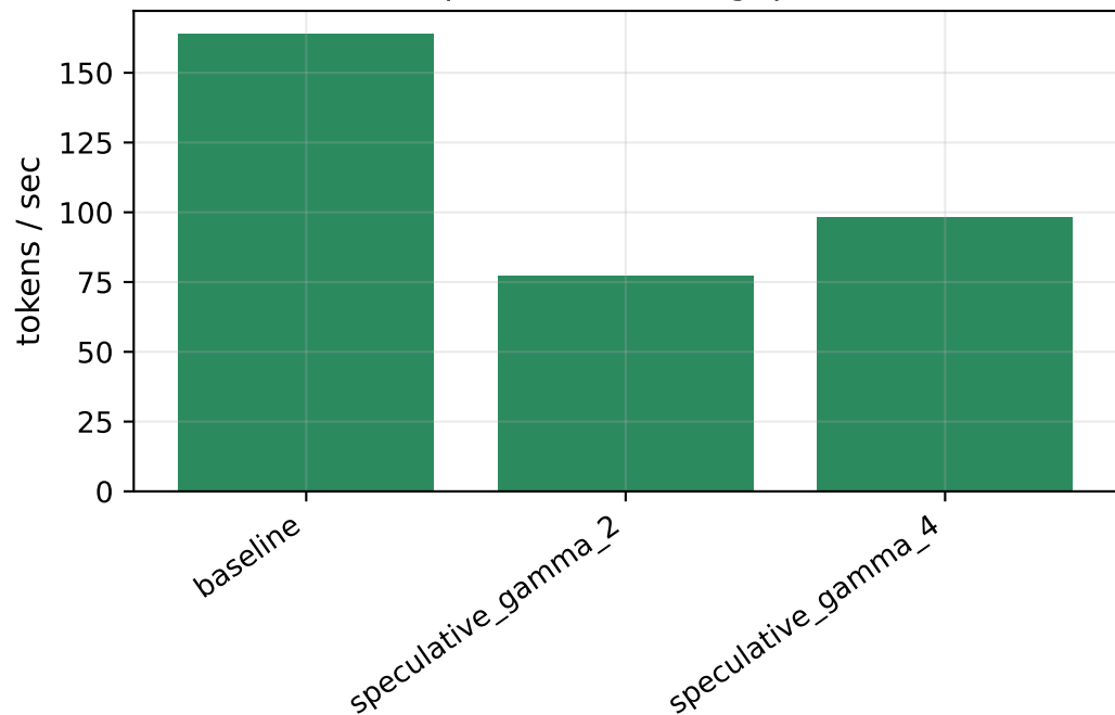
Speculative throughput
