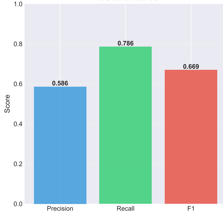
ROUGE-2 Metrics
