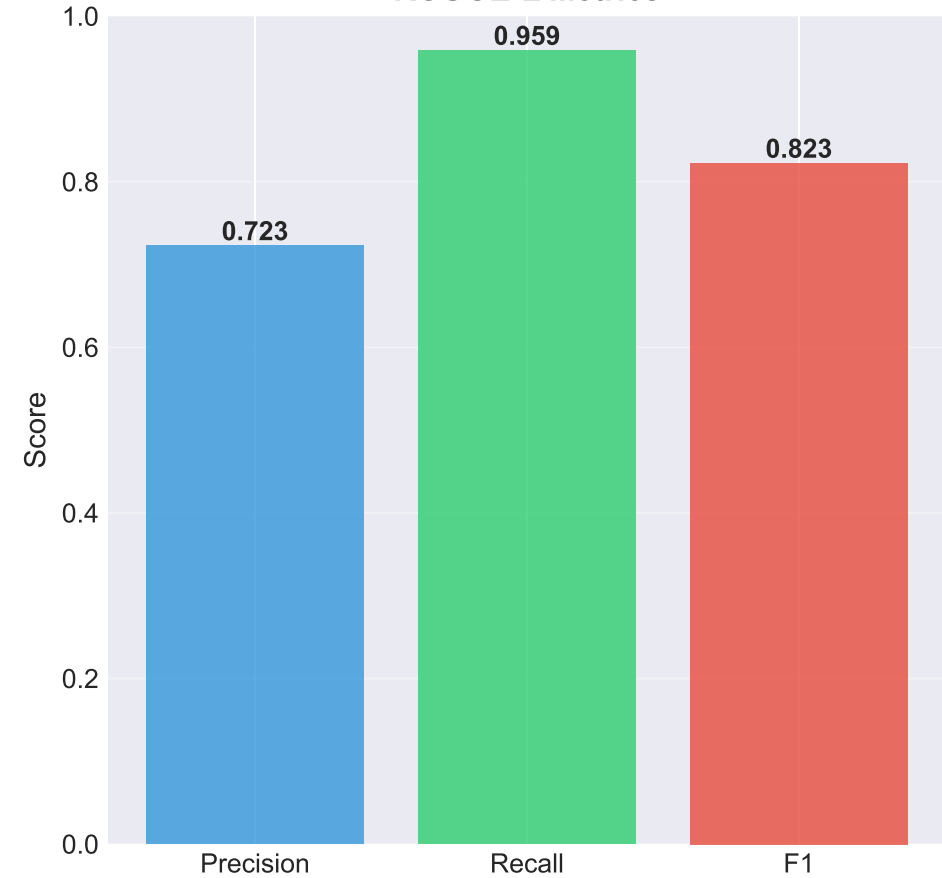
ROUGE-L Metrics
