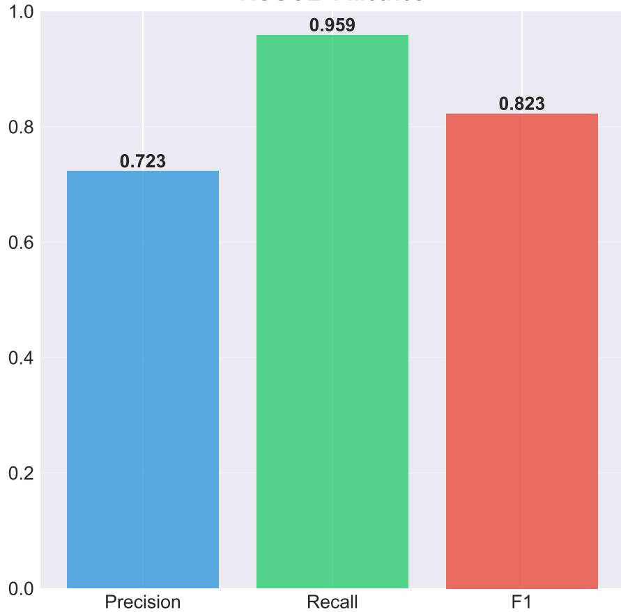
ROUGE-1 Metrics
