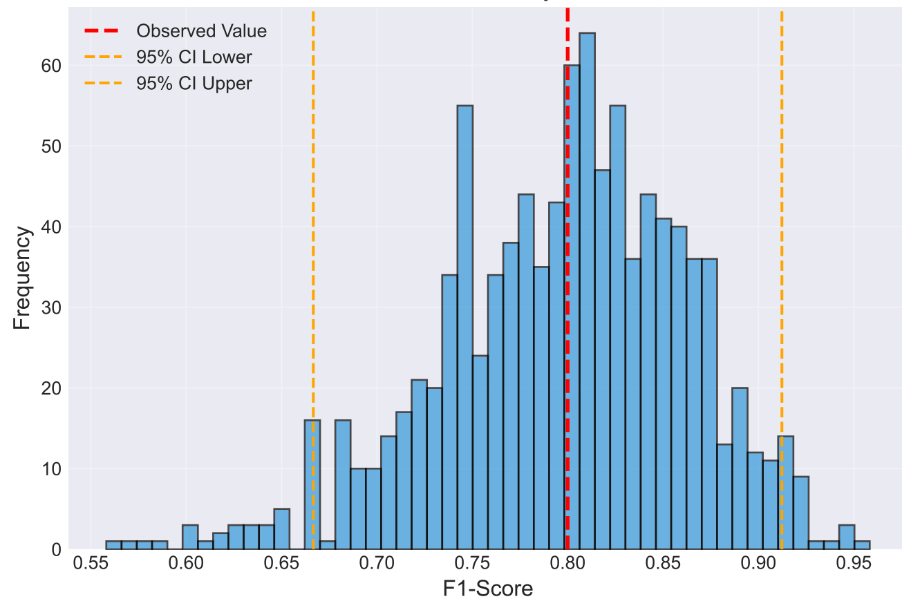
SBD F1-Score Bootstrap Distribution
