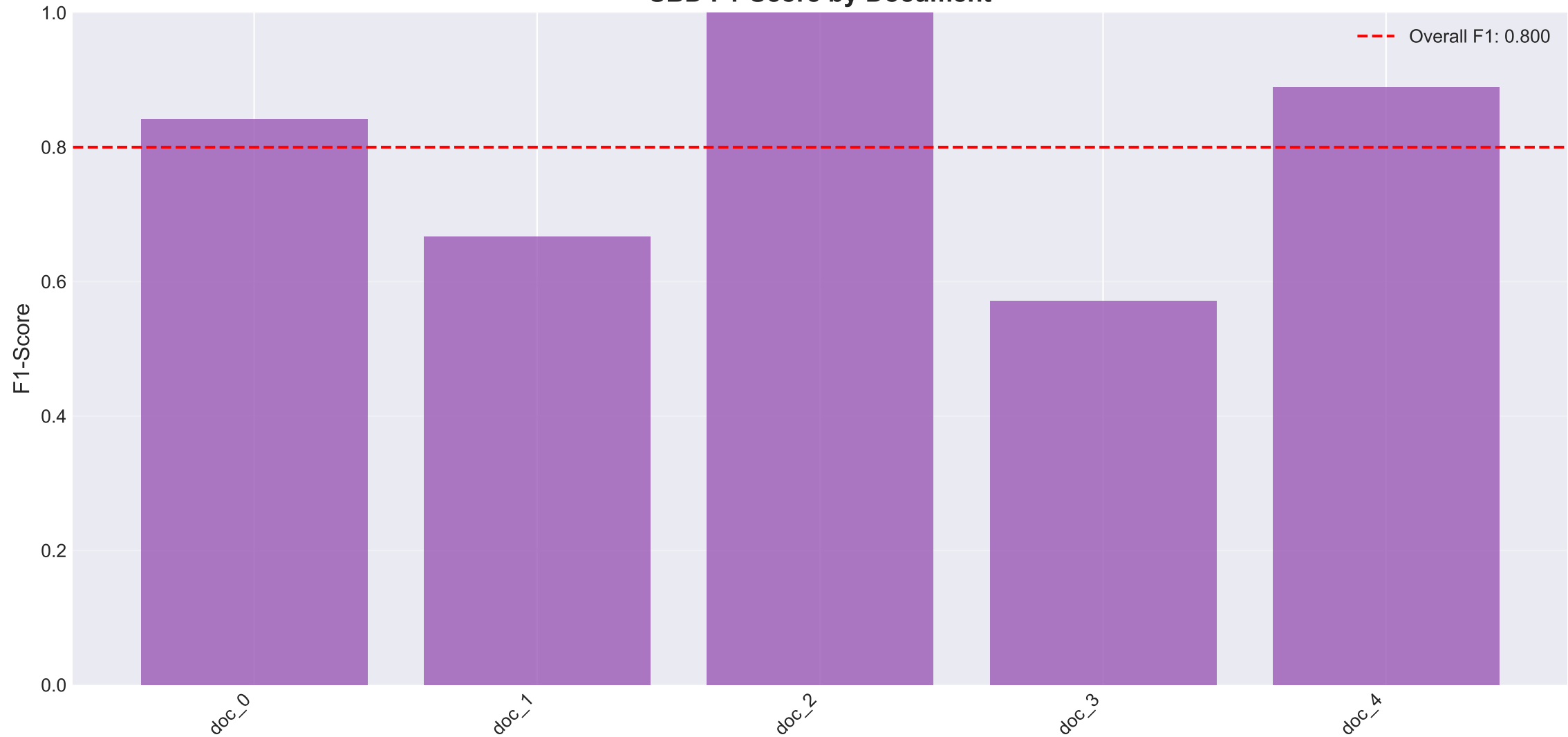
SBD F1-Score by Document
