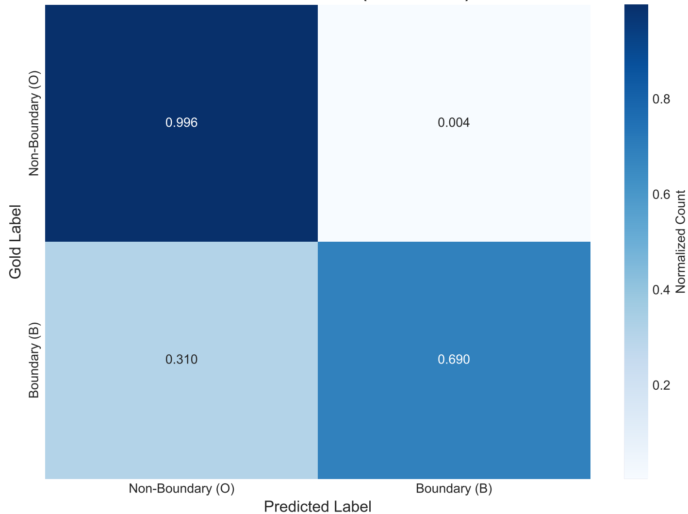
SBD Confusion Matrix (Normalized)
