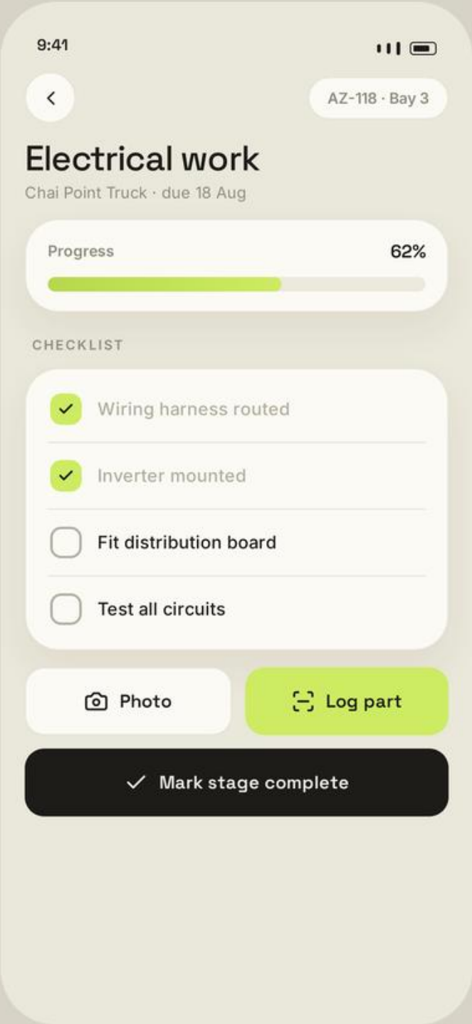
2. Task detail
