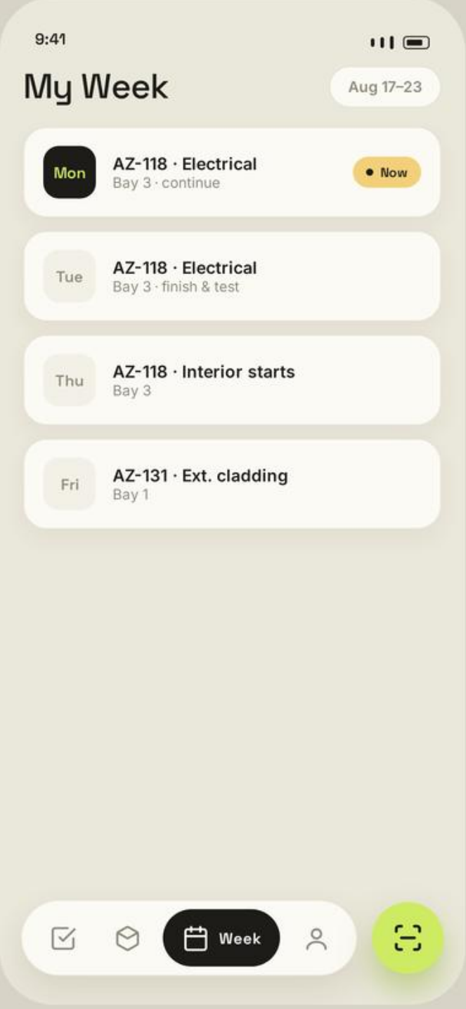
7. My week
