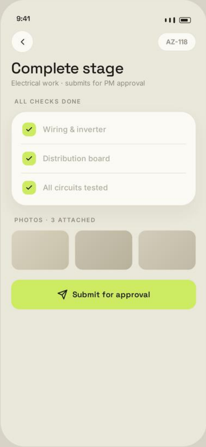
6. Mark complete
