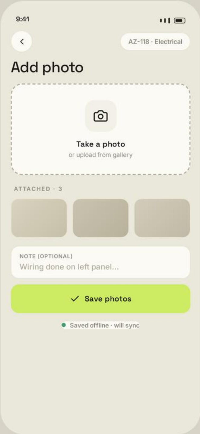
3. Add photo
