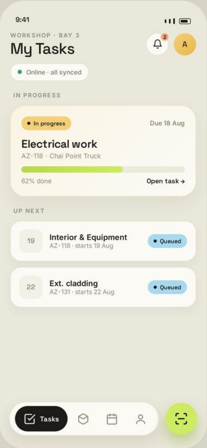
1. My Tasks
