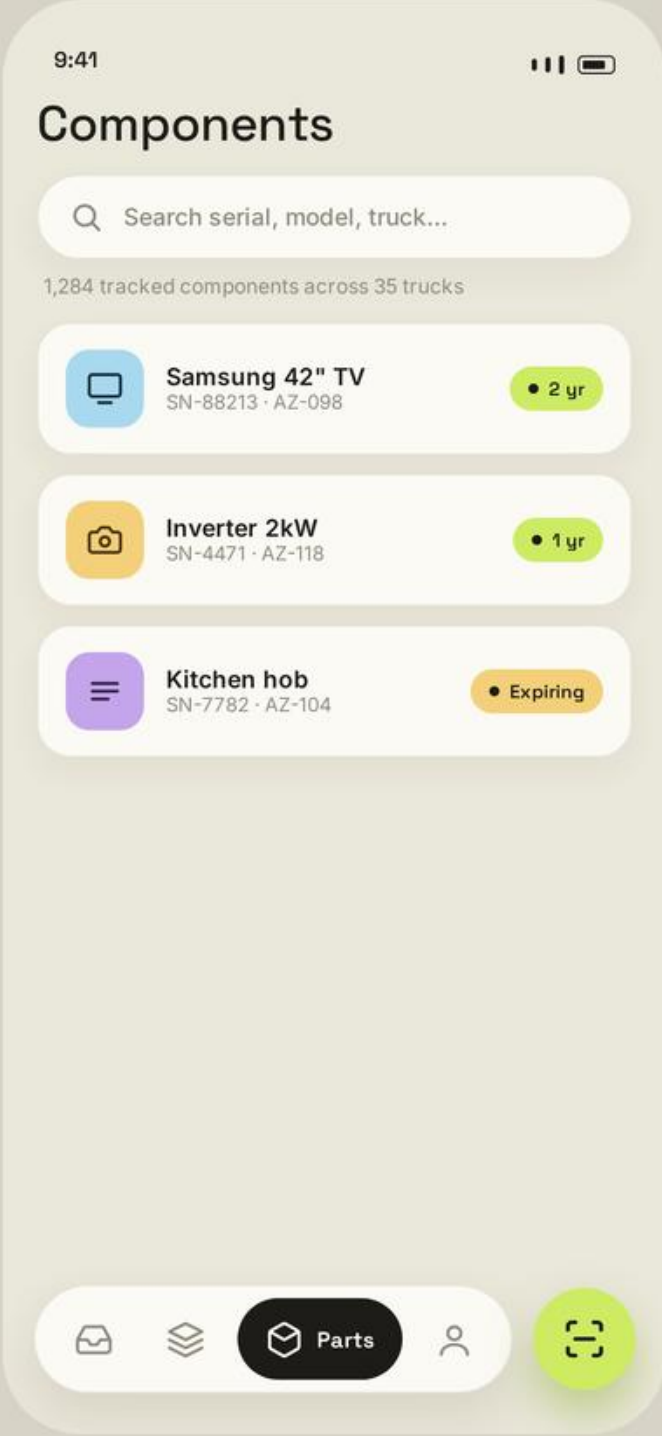
5. Components
