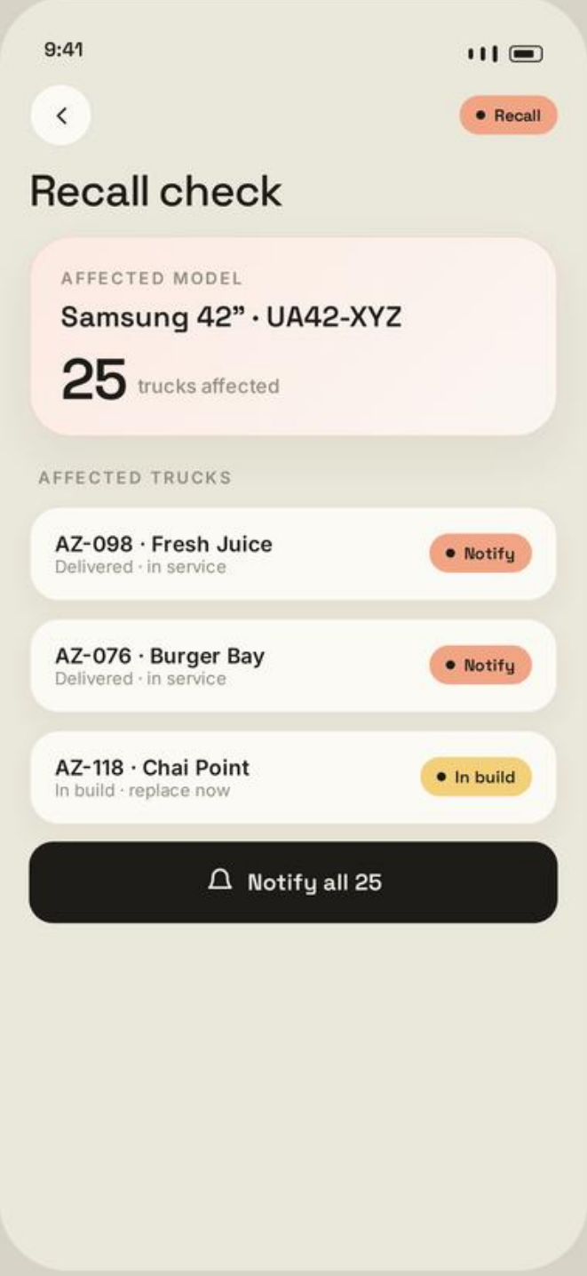
7. Recall check
