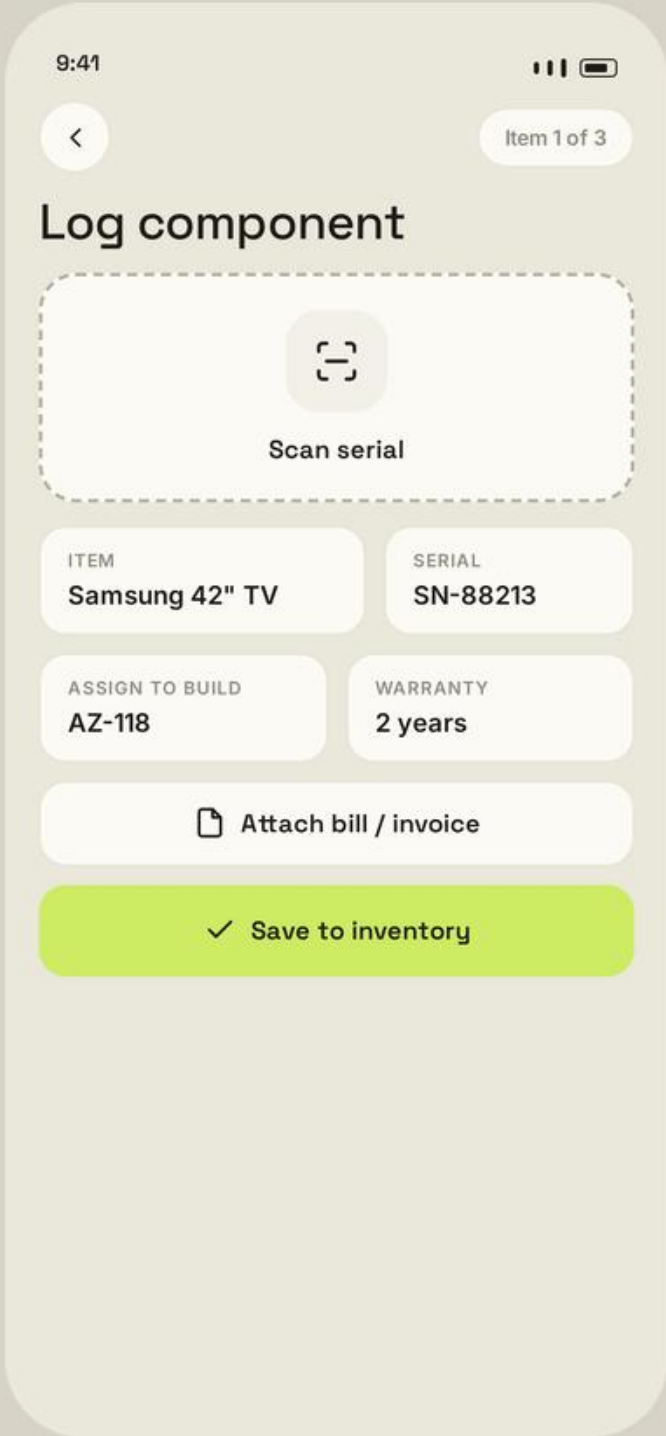
3. Log component
