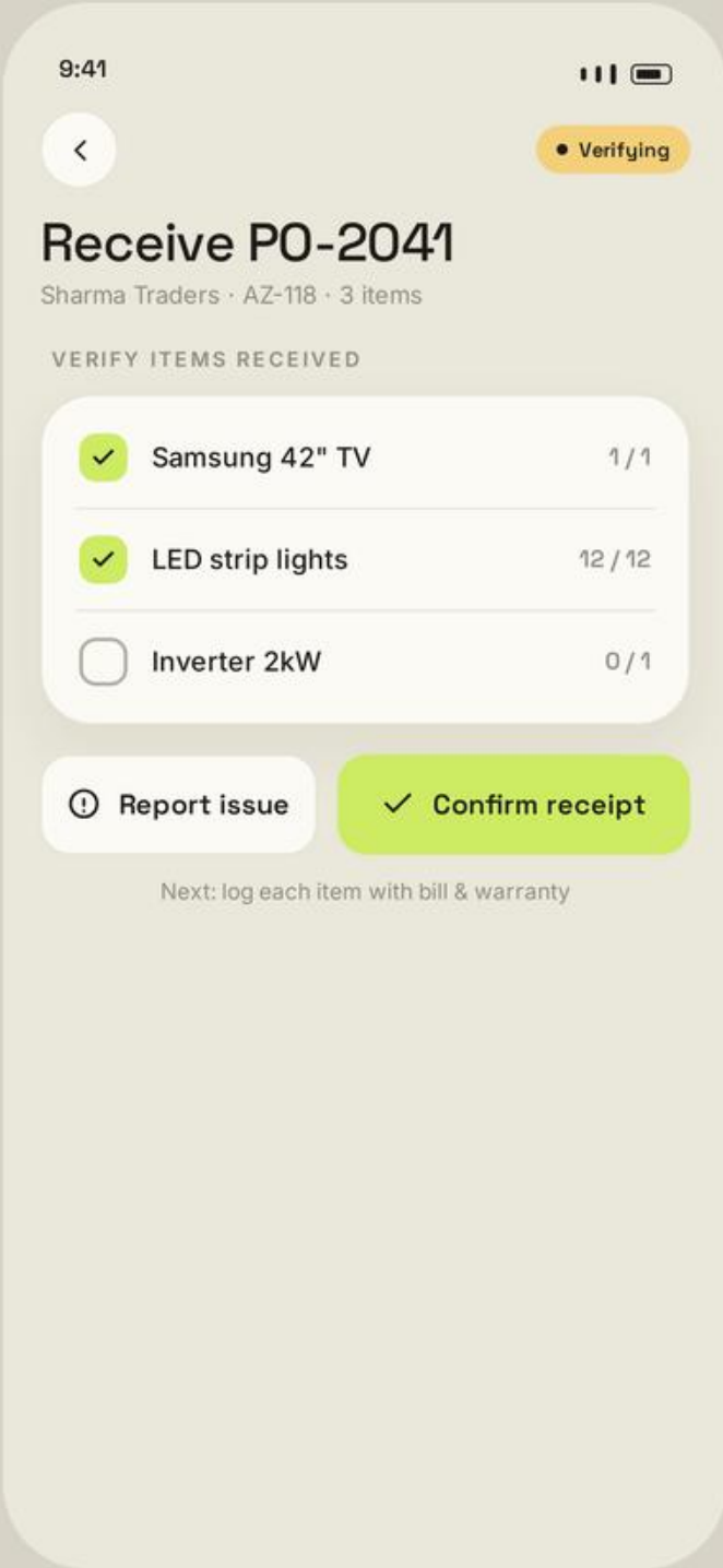
2. Receive / GRN
