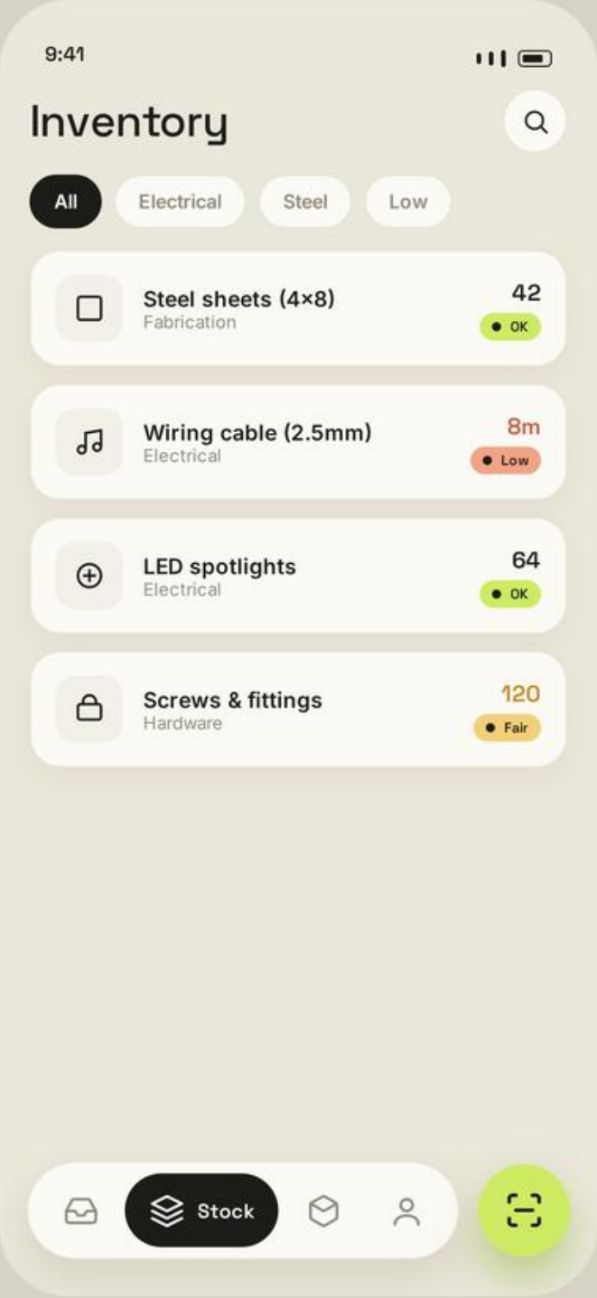
4. Inventory
