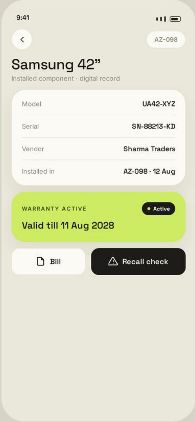
6. Component detail
