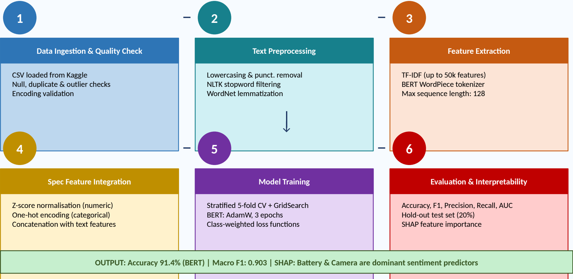
Fig. 3. Six-stage methodology pipeline for five-class sentiment classification of mobile device reviews using the Mobile Reviews Dataset (2025 Edition) [14]
