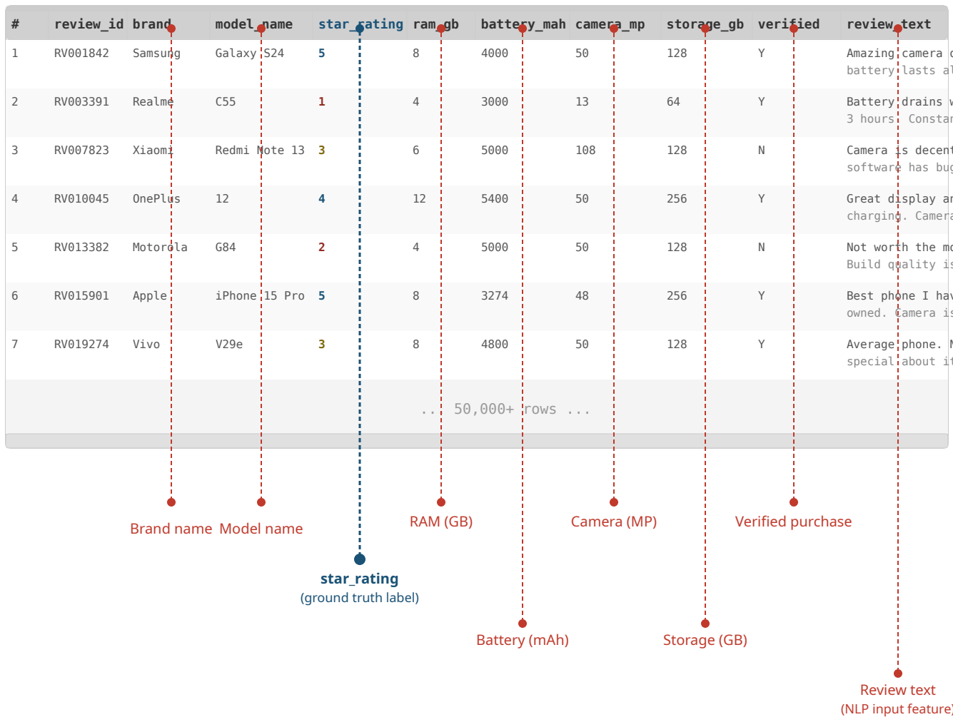
Fig. 2. A screenshot of the captured data from the Mobile Reviews Sentiment and Specification Dataset (2025 Edition) [14].
