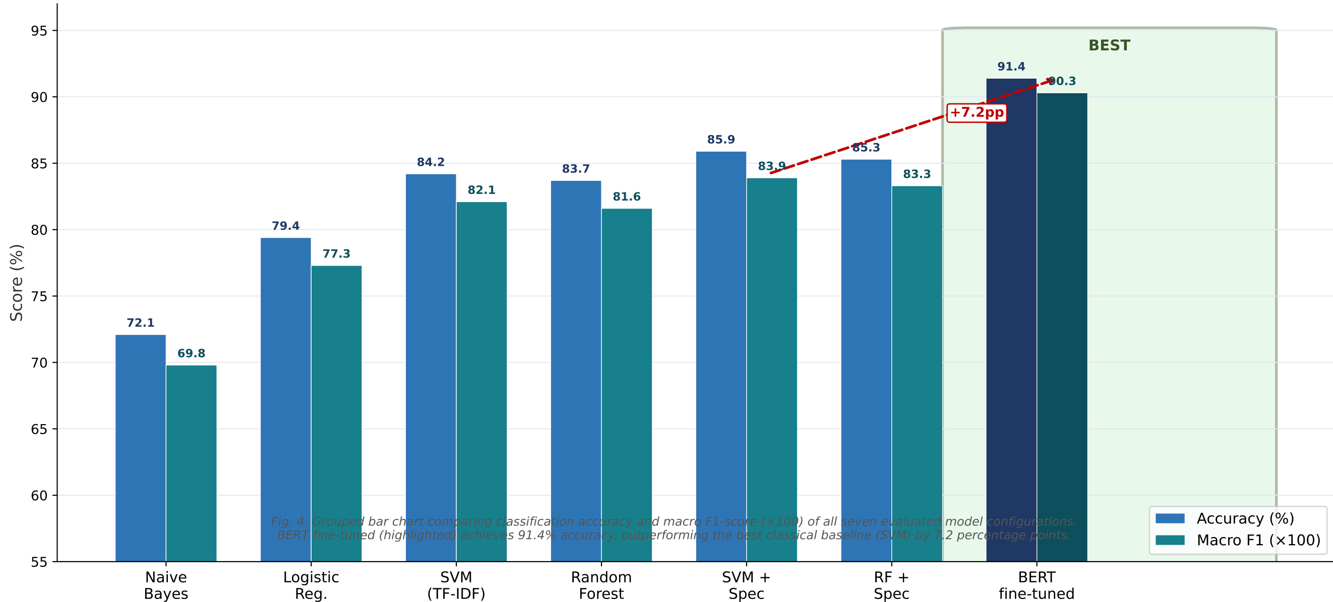
Fig. 4 — Model Performance Comparison: Accuracy and Macro F1-Score Mobile Reviews Sentiment Dataset (2025 Edition) [14]
