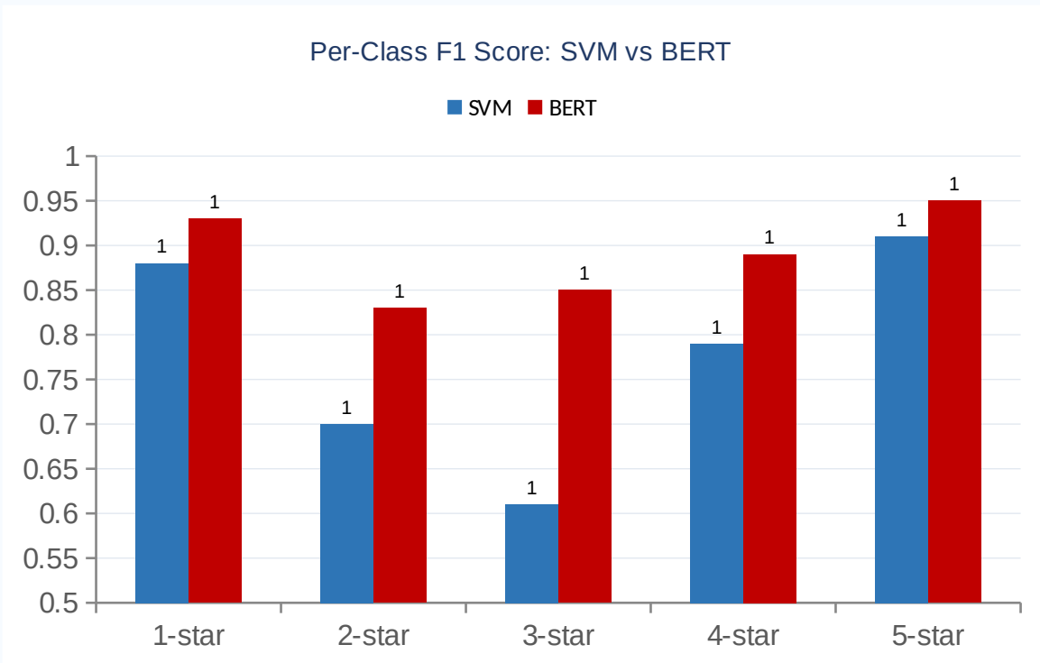
Fig. 5. Per-class F1-score comparison between SVM (best classical) and fine-tuned BERT on all five rating categories. BERT outperforms SVM most significantly on the neutral 3-star class (+23.5 percentage points).
