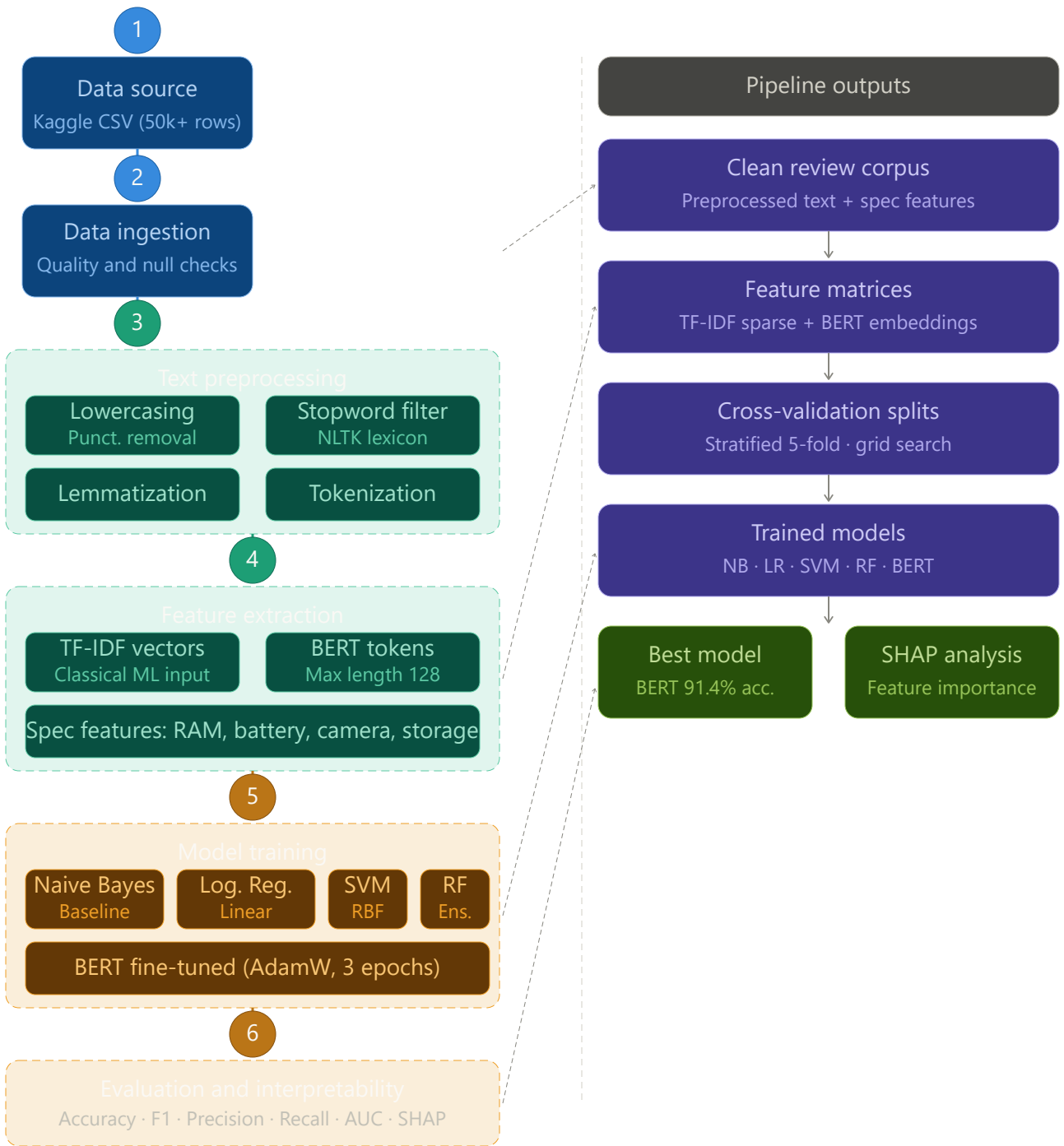
Fig. 3. Flowchart of the proposed six-stage sentiment classification pipeline applied to the Mobile Reviews Dataset (2025 Edition) [14].
