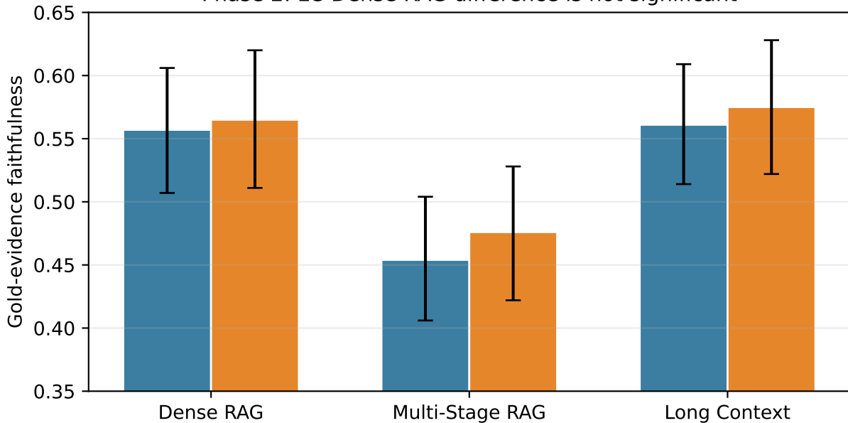
Gemini 2.5 Flash GPT-4o Mini Phase 2: LC-Dense RAG difference is not significant
