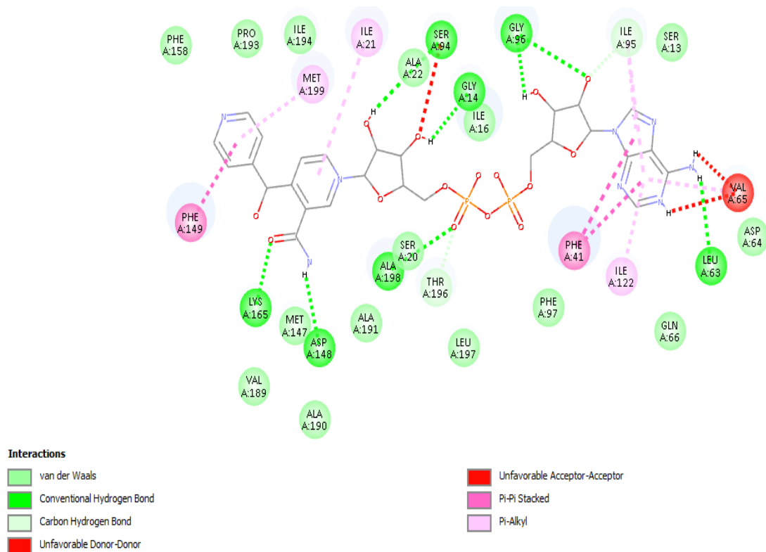
Figure 5. Y158F mutant docked with the INH-NAD adduct. Best pose (-9.5 kcal/mol), equal to wild type.
