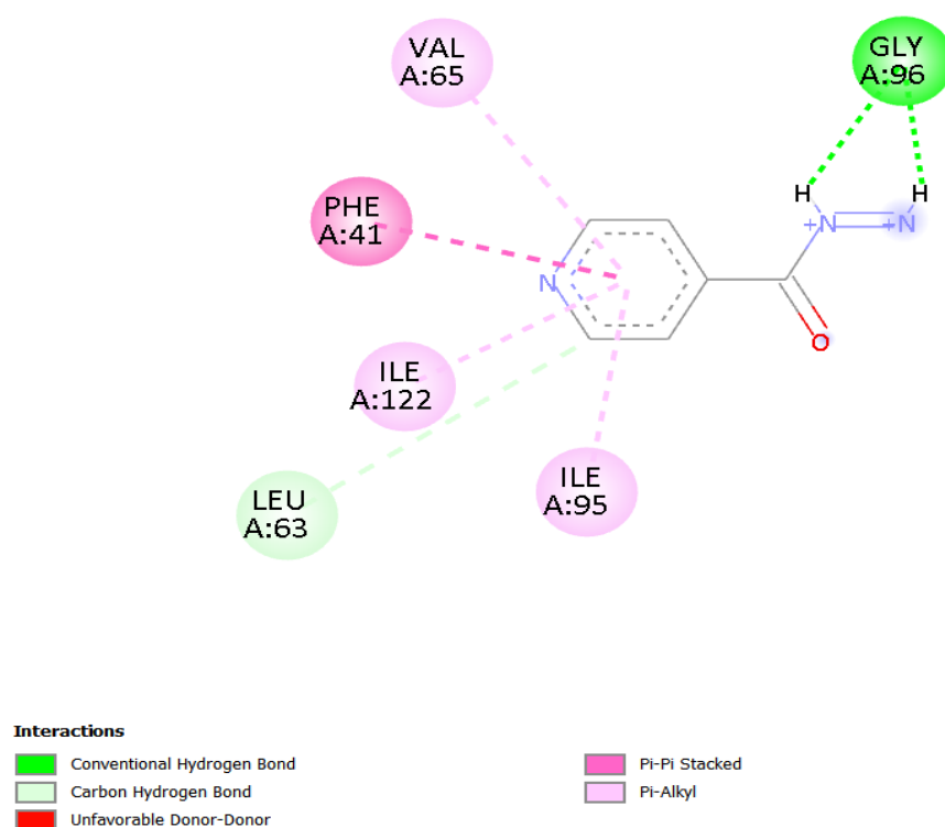
Figure 1. Wild-type InhA docked with isoniazid (INH). Best pose (-5.8 kcal/mol) in the binding pocket; contacting residues: Val65, Leu63, Ile95, Ile122, Phe41, Gly96.
