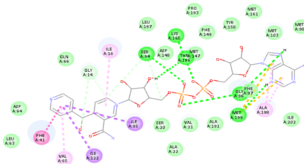
Figure 3. S94A mutant docked with the INH-NAD adduct. Best pose (-10.1 kcal/mol), the strongest predicted binding among all variants.
