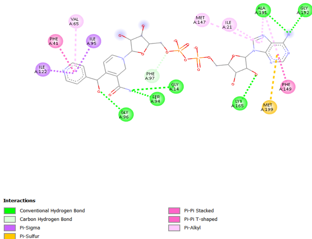
Figure 2. Wild-type InhA docked with the INH-NAD adduct. Best pose (-10.2 kcal/mol) with the 15 contacting residues listed in Section 6.1.
