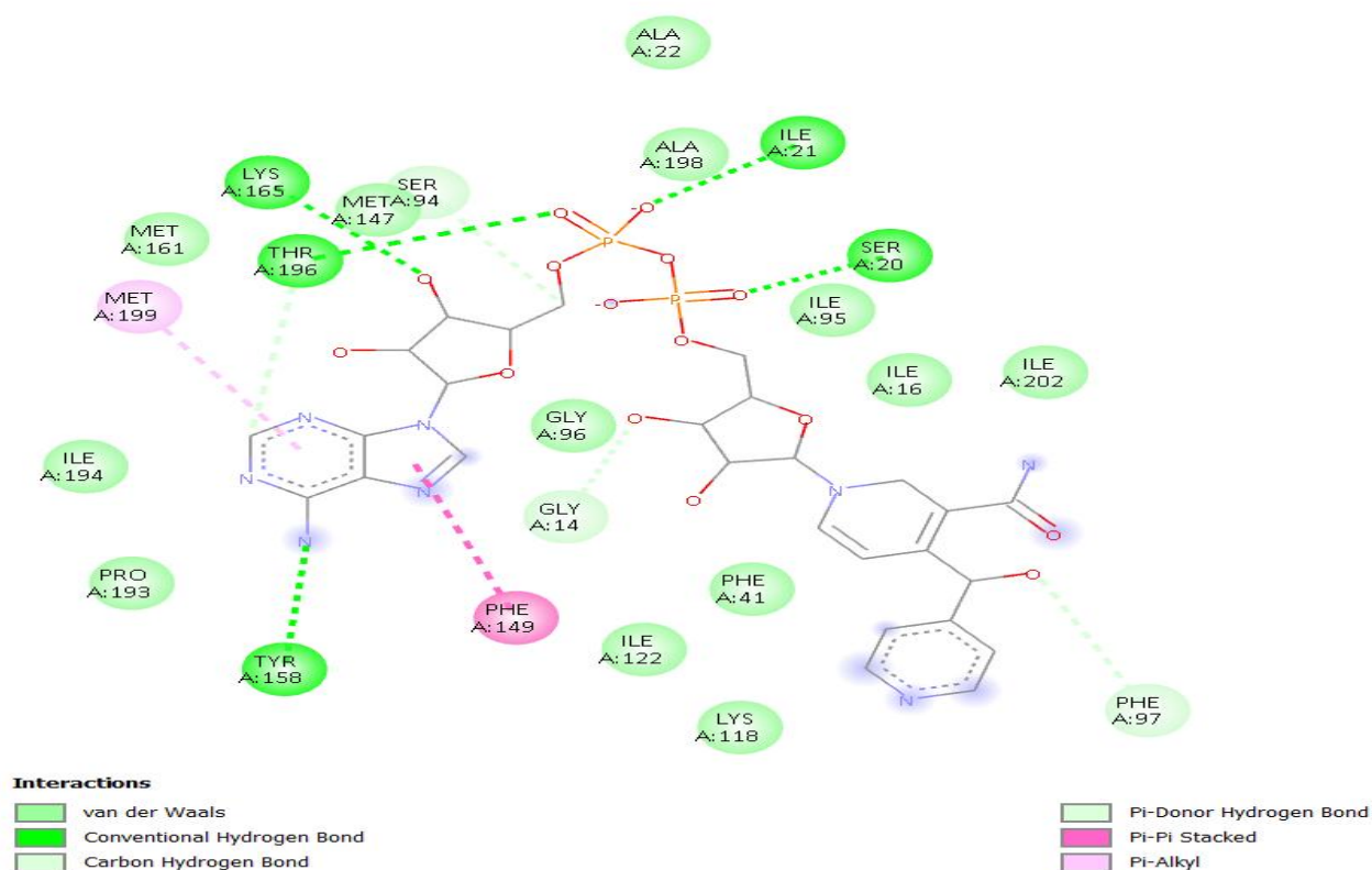
Figure 7. T2A mutant docked with the INH-NAD adduct. Best pose (-10 kcal/mol), the weakest among all variants.
