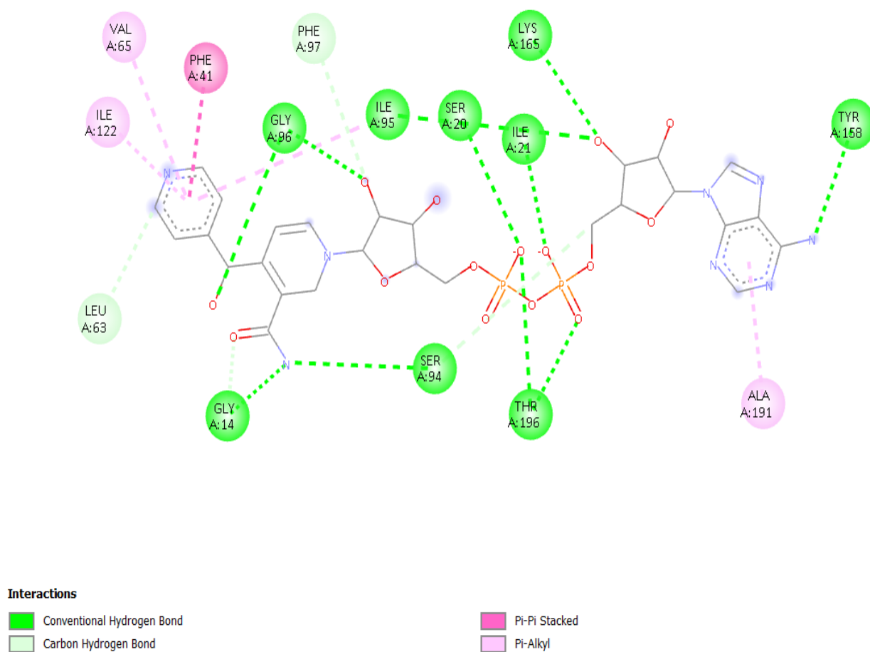
Figure 6. D148G mutant docked with the INH-NAD adduct. Best pose (-11.1 kcal/mol).
