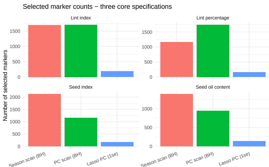
Figure 8. Number of markers selected by the three core model specifications across the four traits.
