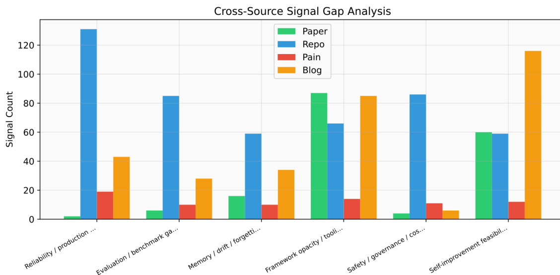
Figure 17: Cross-source validation gap. The survey distinguishes paper claims, open-source implementation evidence, user pain points, and public propagation signals so benchmark gains do not become the only evidence channel.
