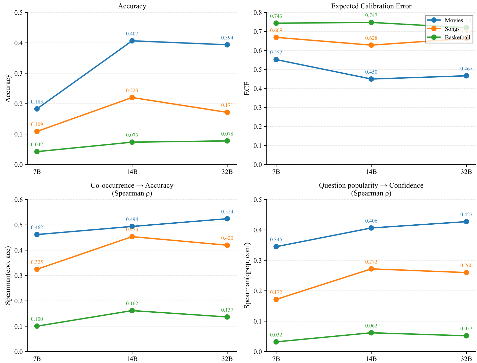
Figure 3: Scaling Does Not Reduce Popularity Bias
