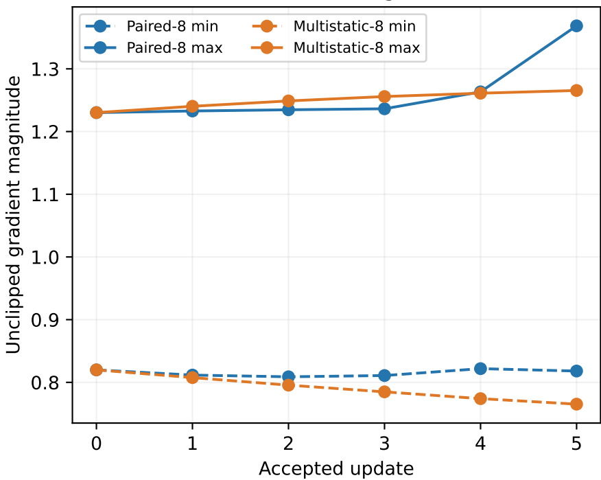
On-contour field gradient
