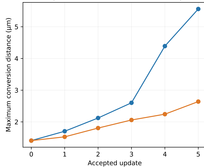
Accepted conversion error (limit: 200 \mu\text{m} )
