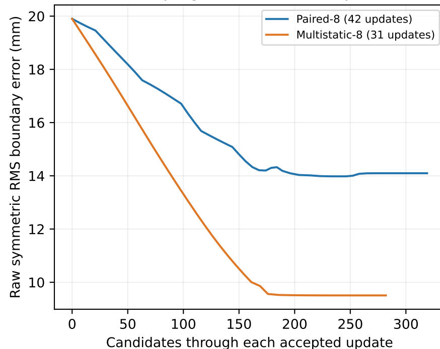
On-contour gradient conditioning
