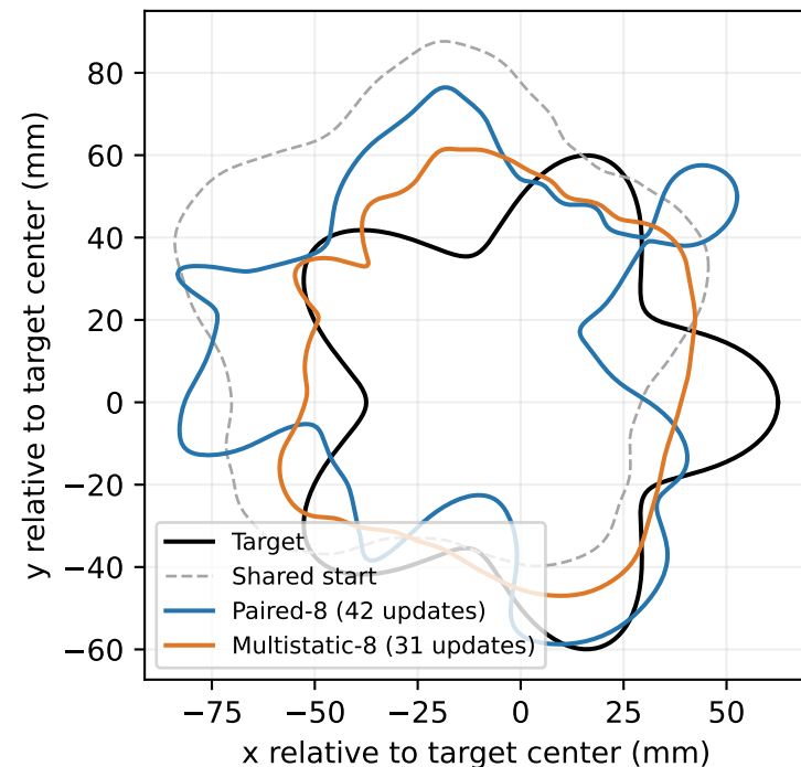
Five-lobe amplitude remains unrecovered
