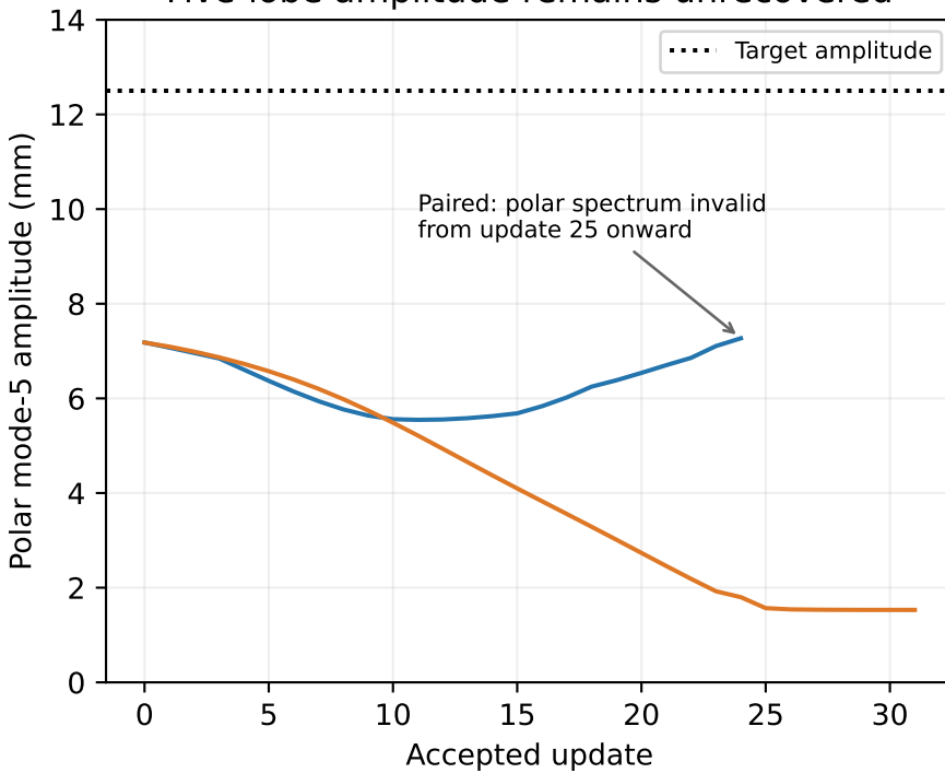
Five-lobe amplitude remains unrecovered
