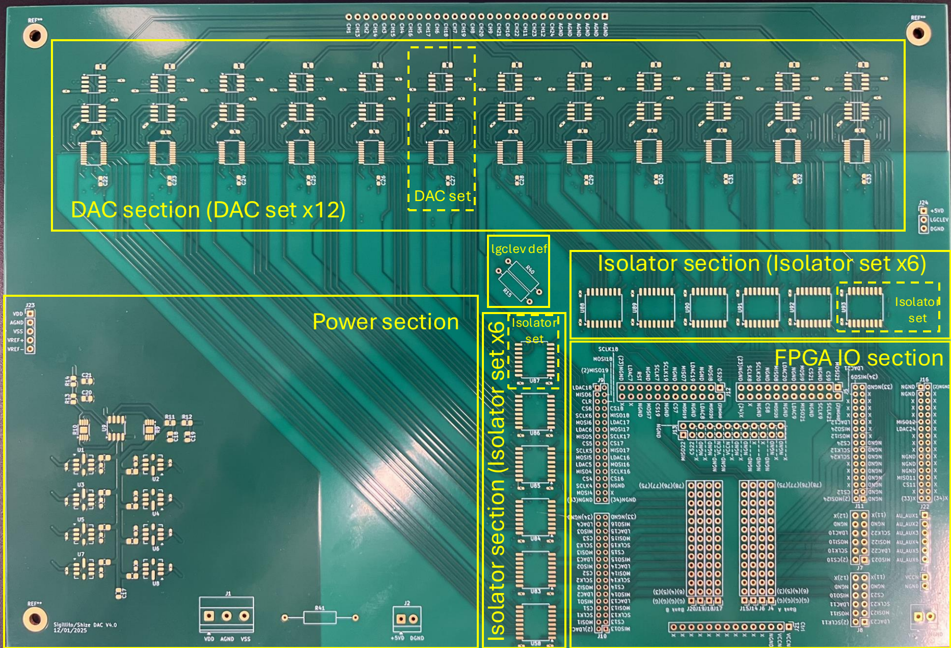
Board front
