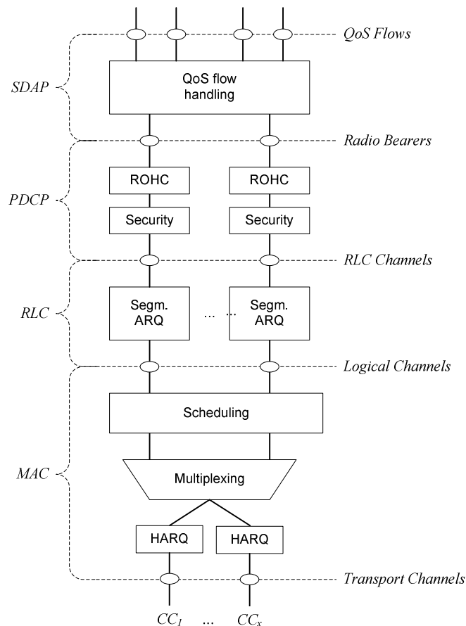
Figure 6.7-2: Layer 2 Structure for UL with CA configured
