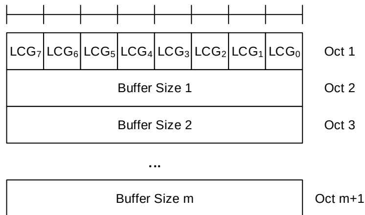
Figure 6.1.3.1-2: Long BSR, Long Truncated BSR, and Pre-emptive BSR MAC CE
