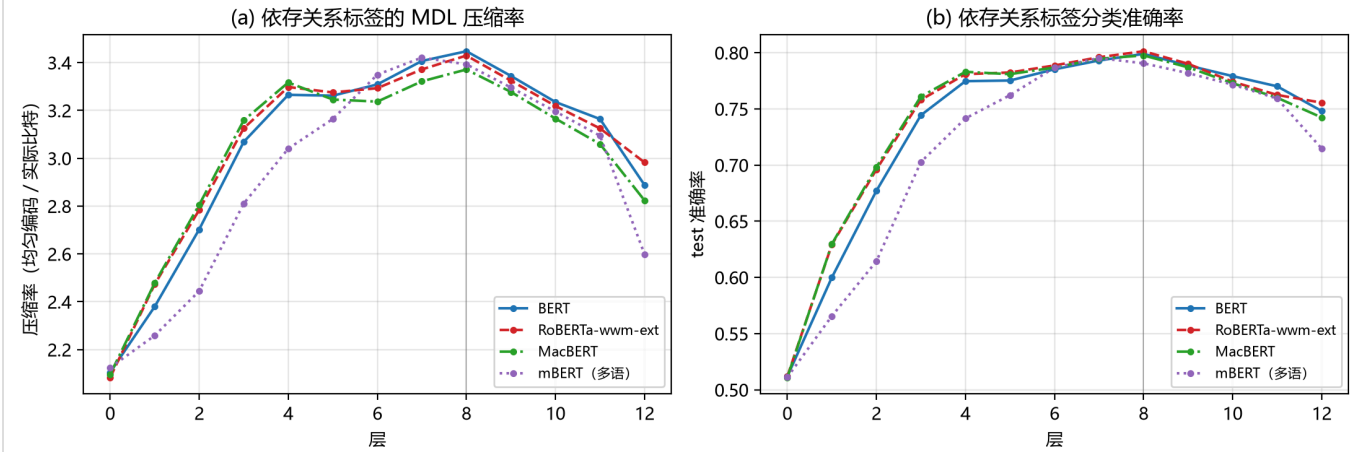
Figure 3 MDL compression ratio and dependency relation classification accuracy (four models)
