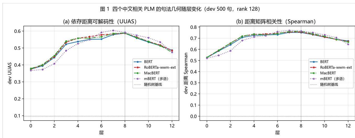
Figure 1 UUAS / distance Spearman curves for four models across 13 layers (with the random-tree baseline)
