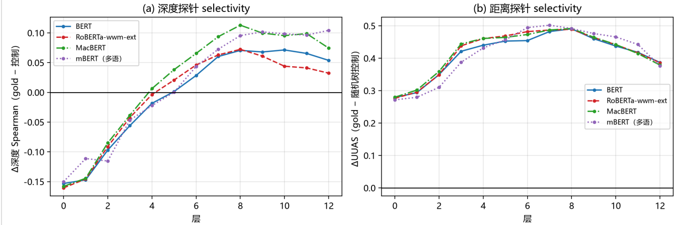
Figure 2 selectivity as a function of layer (depth / distance, four models)
