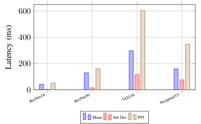
Fig. 7. Latency statistics observed across the evaluated architectures.
