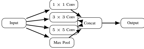
Fig. 3. Simplified Inception-style multi-branch module with concatenation merge.
