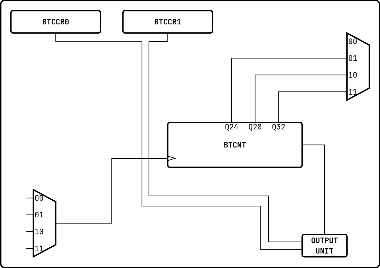
Timer Core
