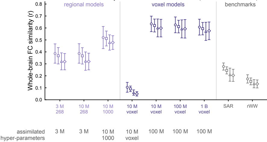
Whole-brain FC similarity: DTB builds vs benchmarks (mean \pm s.d., n = 12)
