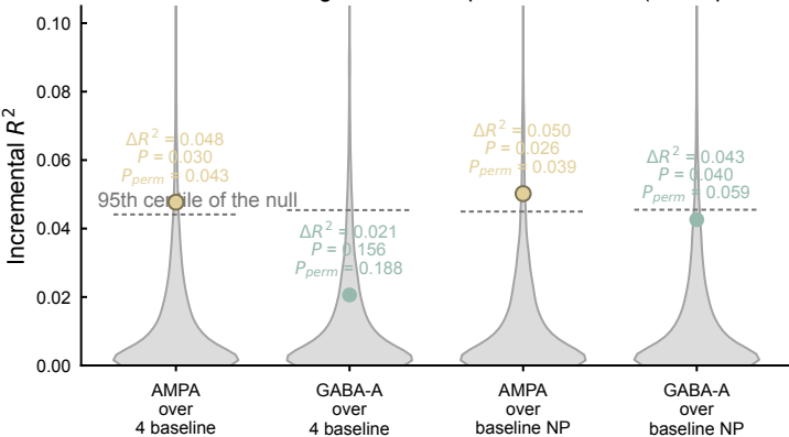
Incremental variance against its own permutation null (5,000 permutations of the outcome)
