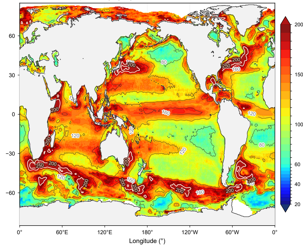
d Rhines scale, \sqrt{2U_{\text{rms}}/\beta} (km)
