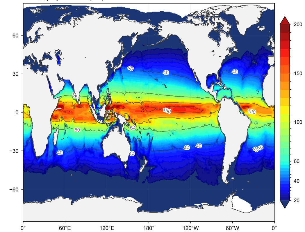
e L_{\text{eddy}} dynamical (km)
