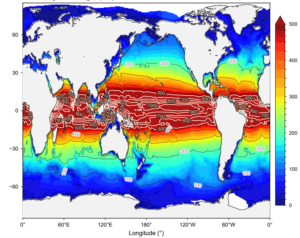
f 2\pi L_{\text{eddy}} wavelength (km)
