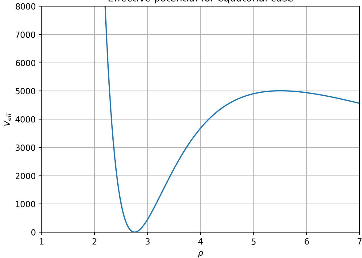
Effective potential for equatorial case
